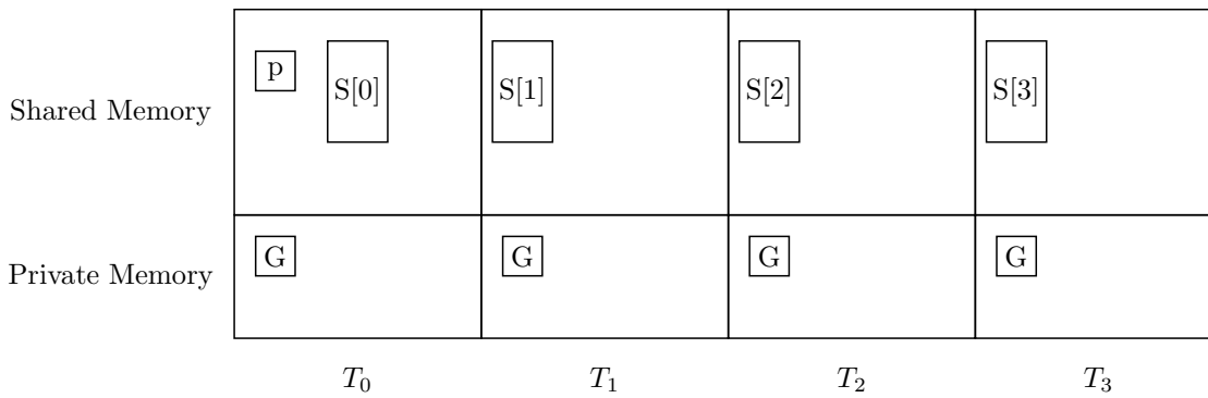
Figure 5: UPC Declarations
