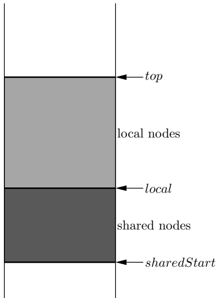
Figure 7: A stack
