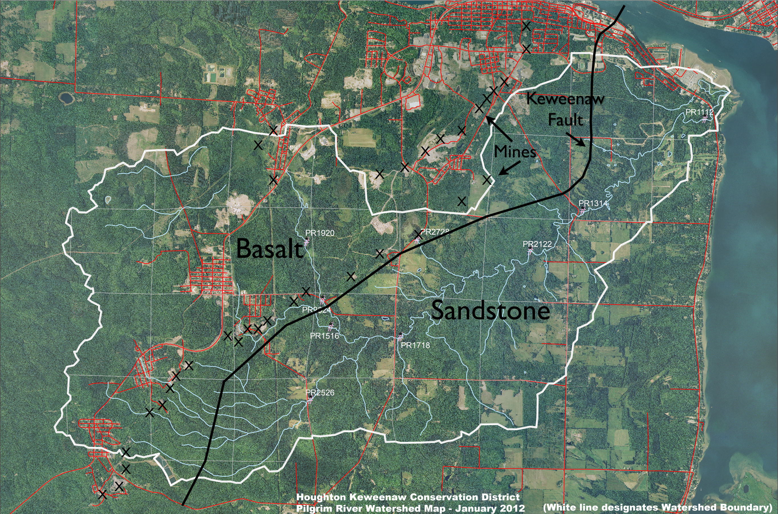
Fig I: Simplified Geologic map of Pilgrim Watershed
