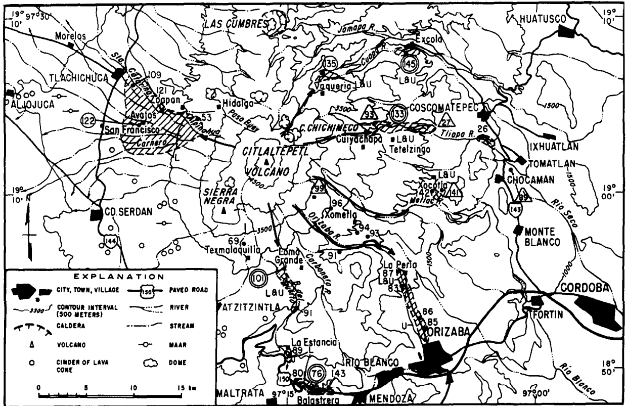
Fig. 2. Distribution map of the Citlaltépetl ignimbrite deposits (diagonals). Arrows indicate suggested flow paths. Numbers indicate sampling sites: circled numbers locate key sections shown in Fig. 4, double circle where ^{14}\text{C} date is available, and triangles for other deposits with ^{14}\text{C} (Table 3). Labels indicate stratigraphic members: L = Lower; U = Upper member; and L&U = both members.
