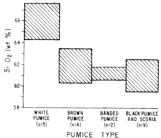
Fig. 7. Silica content ranges for juvenile components in the Citlaltépetl ignimbrite deposit.
