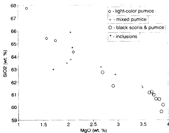
Fig. 9. Plot of wt.% SiO 2 versus MgO for pyroclastic material from Citlaltépetl volcano.
