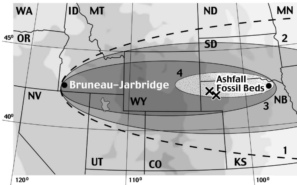
Figure 1. Location map showing Bruneau-Jarbridge volcano in SW Idaho and Ashfall Fossil Beds in NE Nebraska and two sampled ash localities in Morrill County, Western Nebraska (x). Possible ellipsoidal shapes of distal isomass lines on the map are speculatively outlined, by analogy with other well-sampled distal fall deposit maps such as Sarna-Wojcicki et al. (1981) and McGimsey et al. (2001). Ellipsoidal lines 1–3 show the possible configuration of a deposit that exponentially thins away from the source, whereas ellipse 4 outlines a possible “secondary maximum” of deposition, such as that shown by well-mapped deposits.
