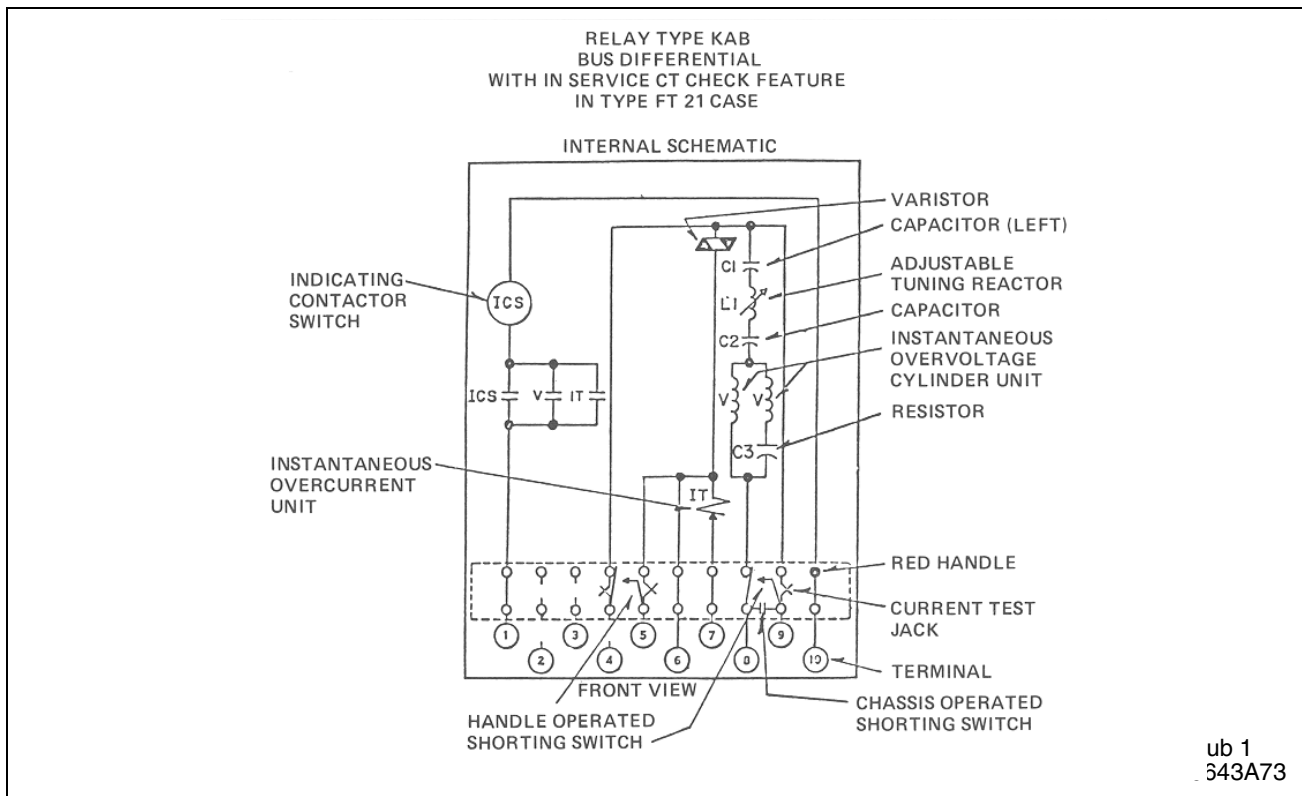
Figure 5. Internal Schematic of KAB RELAY with untapped ICS unit and with in service ct Check Feature.
