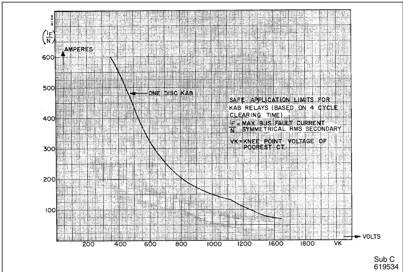
Figure 12. Safe Application Limits for KAB Relays.
