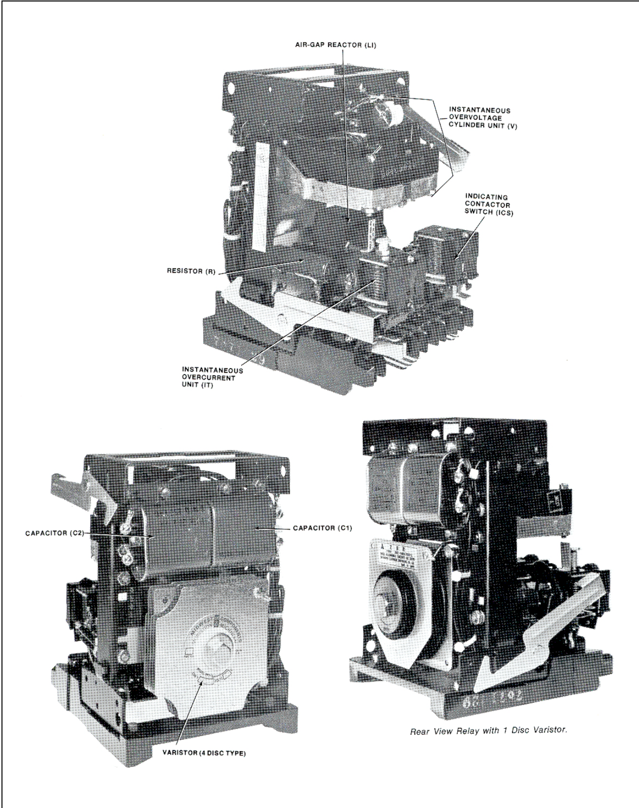
Figure 1. Type KAB Relay Without Case
