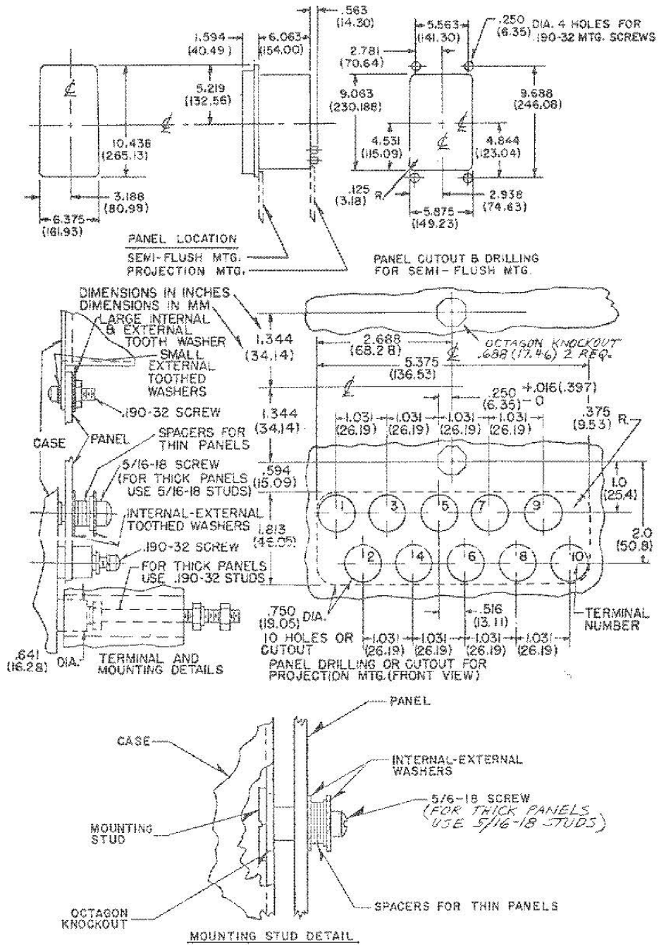
Figure 13. Outline and Drilling Plan For Type KAB Relay In Type FT-21 Case.
