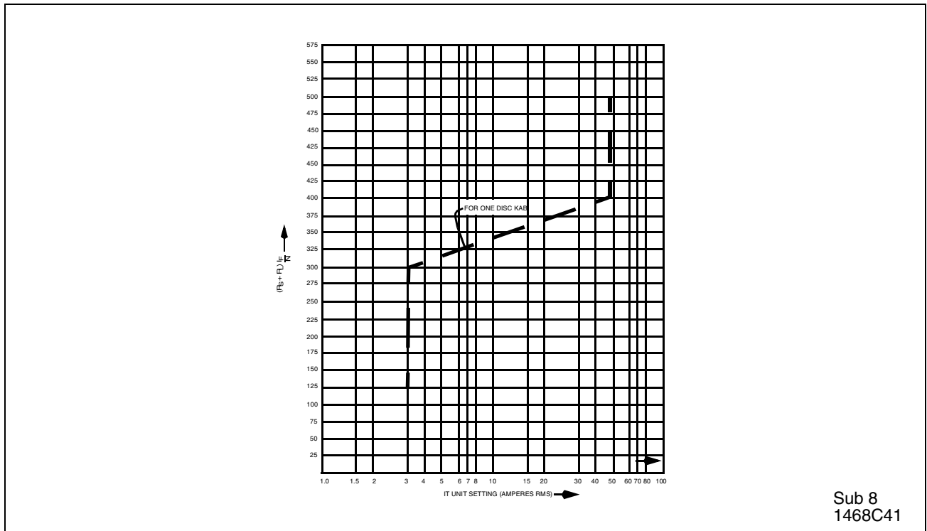
Figure 9. IT Unit Setting.
