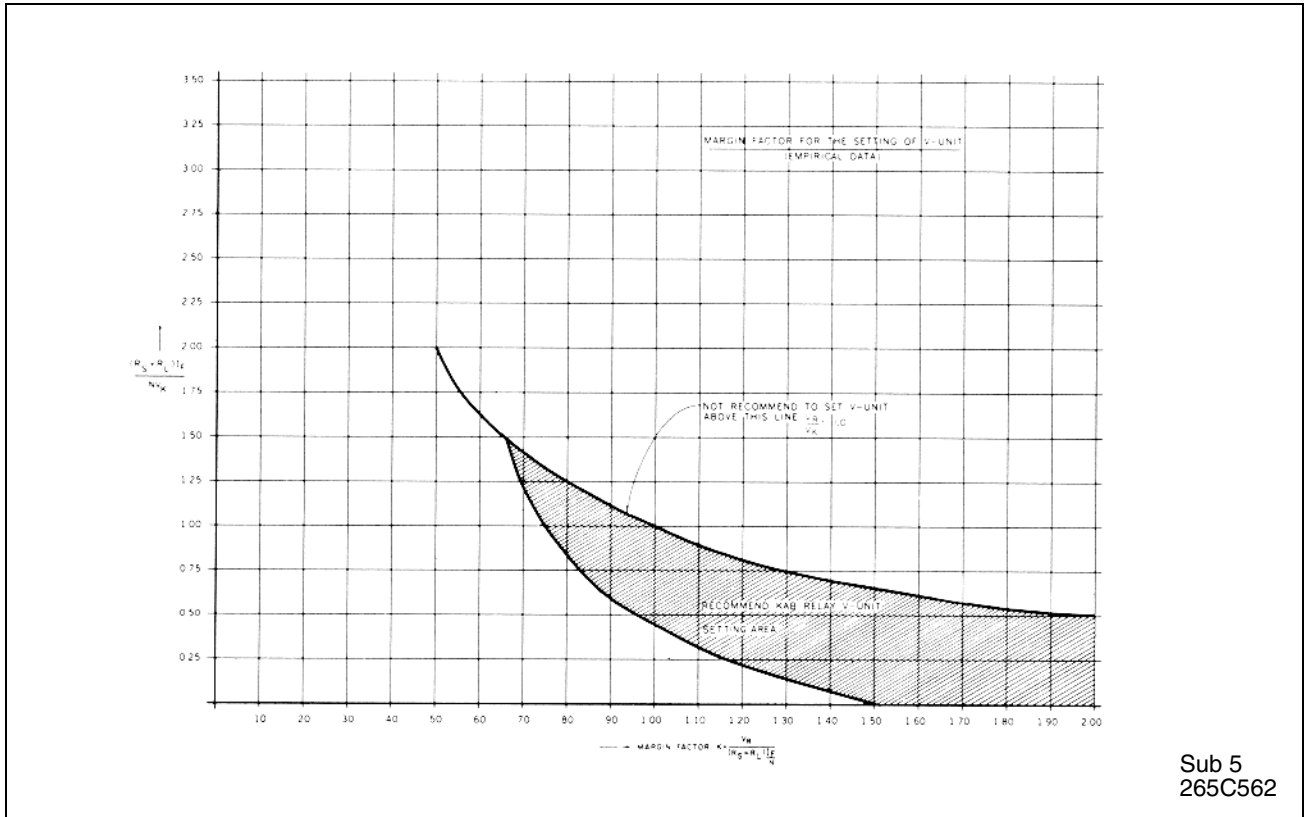
Figure 8. Margin Factor For V-Unit Setting.
