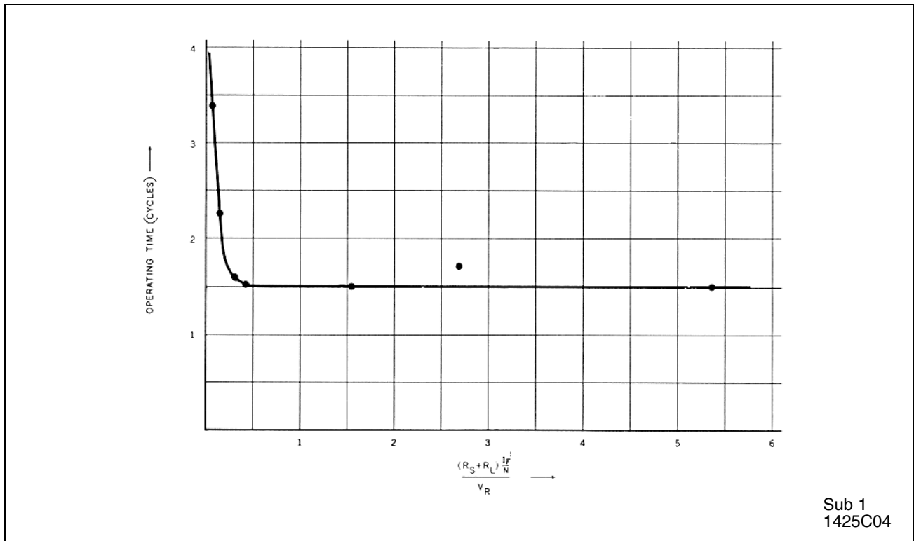
Figure 11. KAB Relay Typical Operating Time (from stage fault tests).
