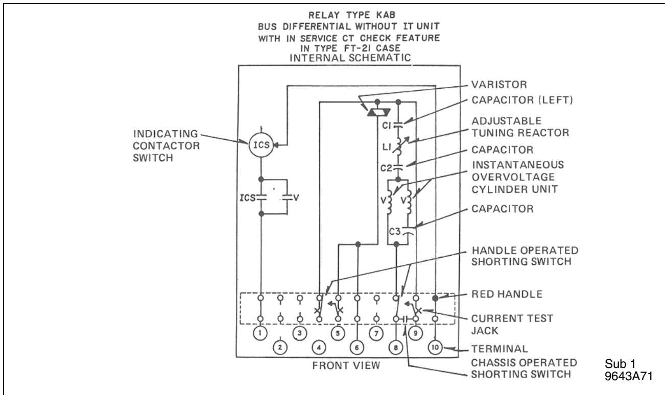
Figure 4. Internal Schematic of KAB Relay without instantaneous overcurrent unit and with in Service ct Check Feature. Pertains to all KAB Relay Style 6668D37A08 and above (without IT unit)
