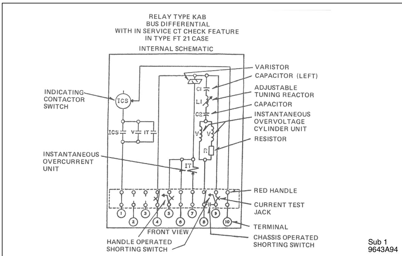
Figure 2. Internal Schematic Of KAB (150-400 Vac) Relay With In Service ct Check Feature.
