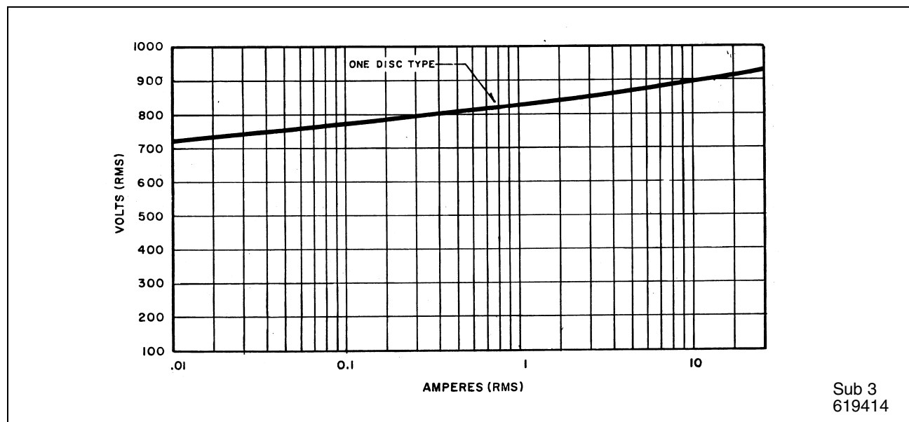
Figure 7. Typical Volt-Ampere Characteristic of Varistor in Type KAB Relay (RMS).
