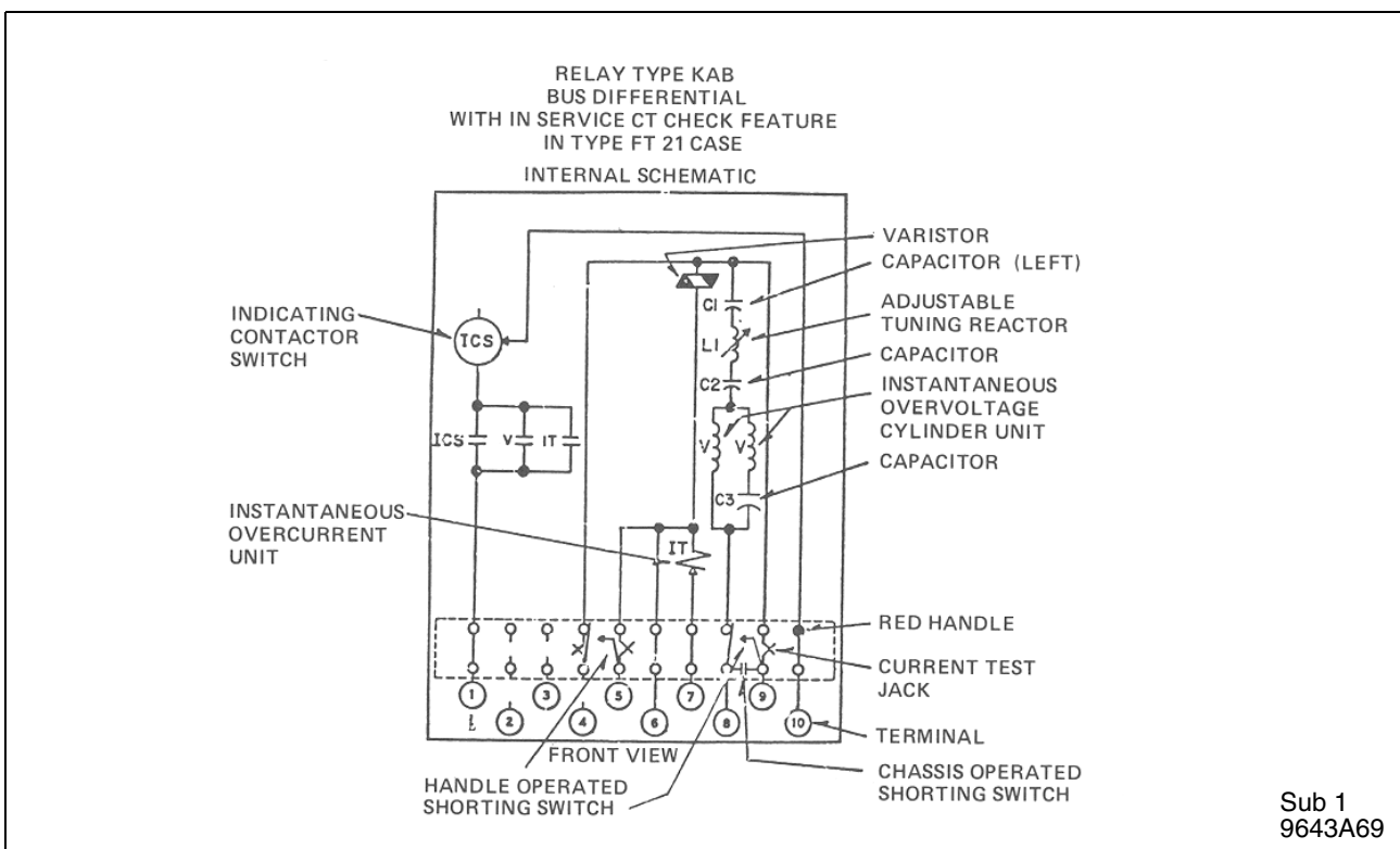
Figure 3. Internal Schematic of KAB Relay with in Service ct Check Feature. Pertains to all KAB Relay Styles 6668D37A04 and above (with IT unit).
