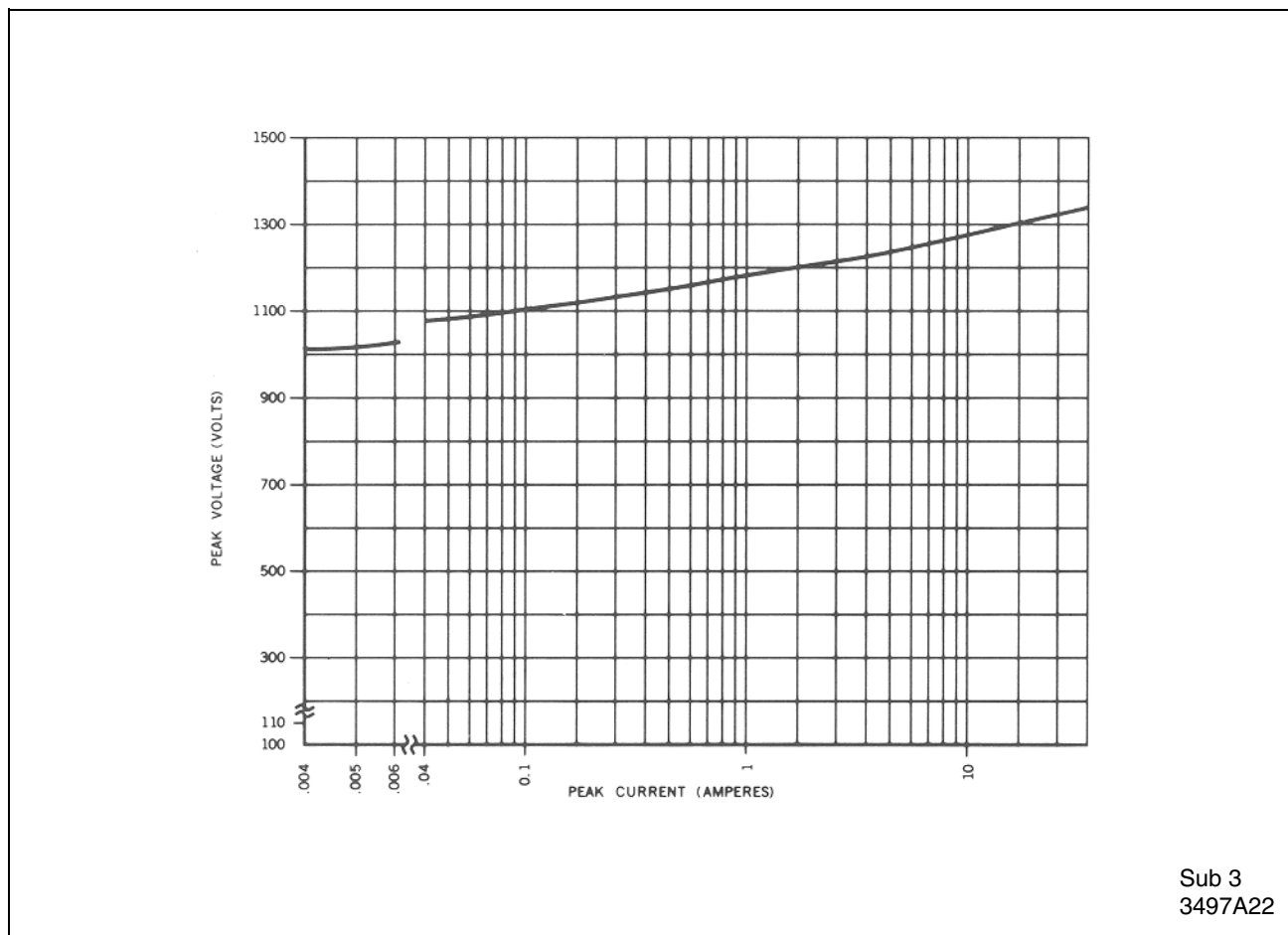
Figure 6. Typical Volt-Ampere Characteristic of Varistor in Type KAB Relay (Peak Value).
