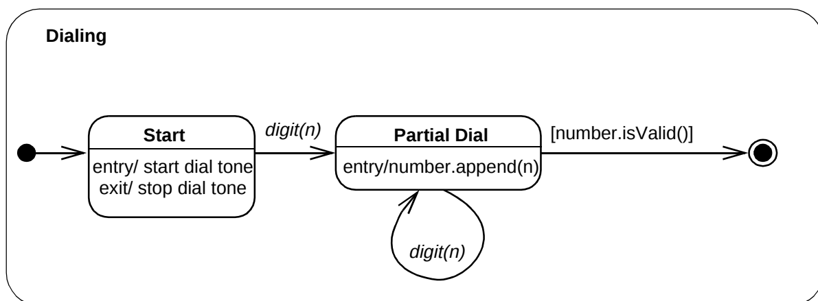
Figure 43. Sequential substates
