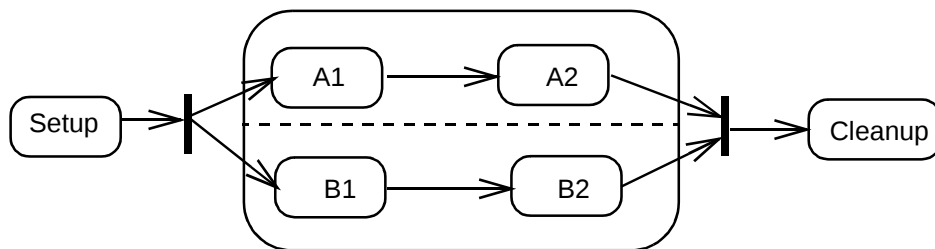
Figure 46. Complex transition
