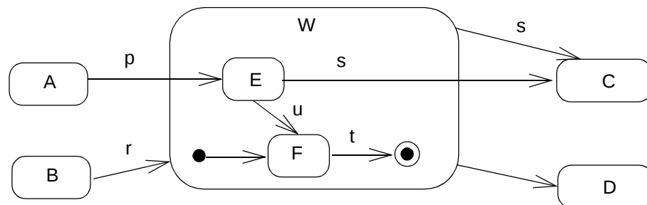
Figure 47. Stubbed transitions
