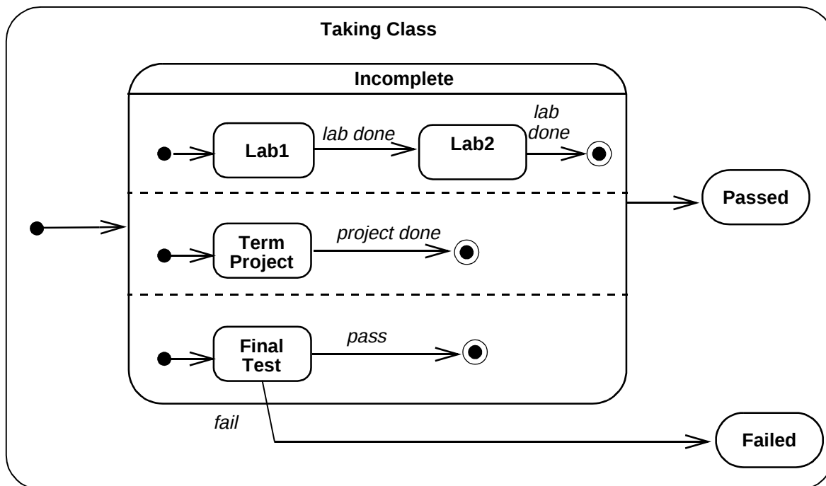
Figure 44. Concurrent substates
