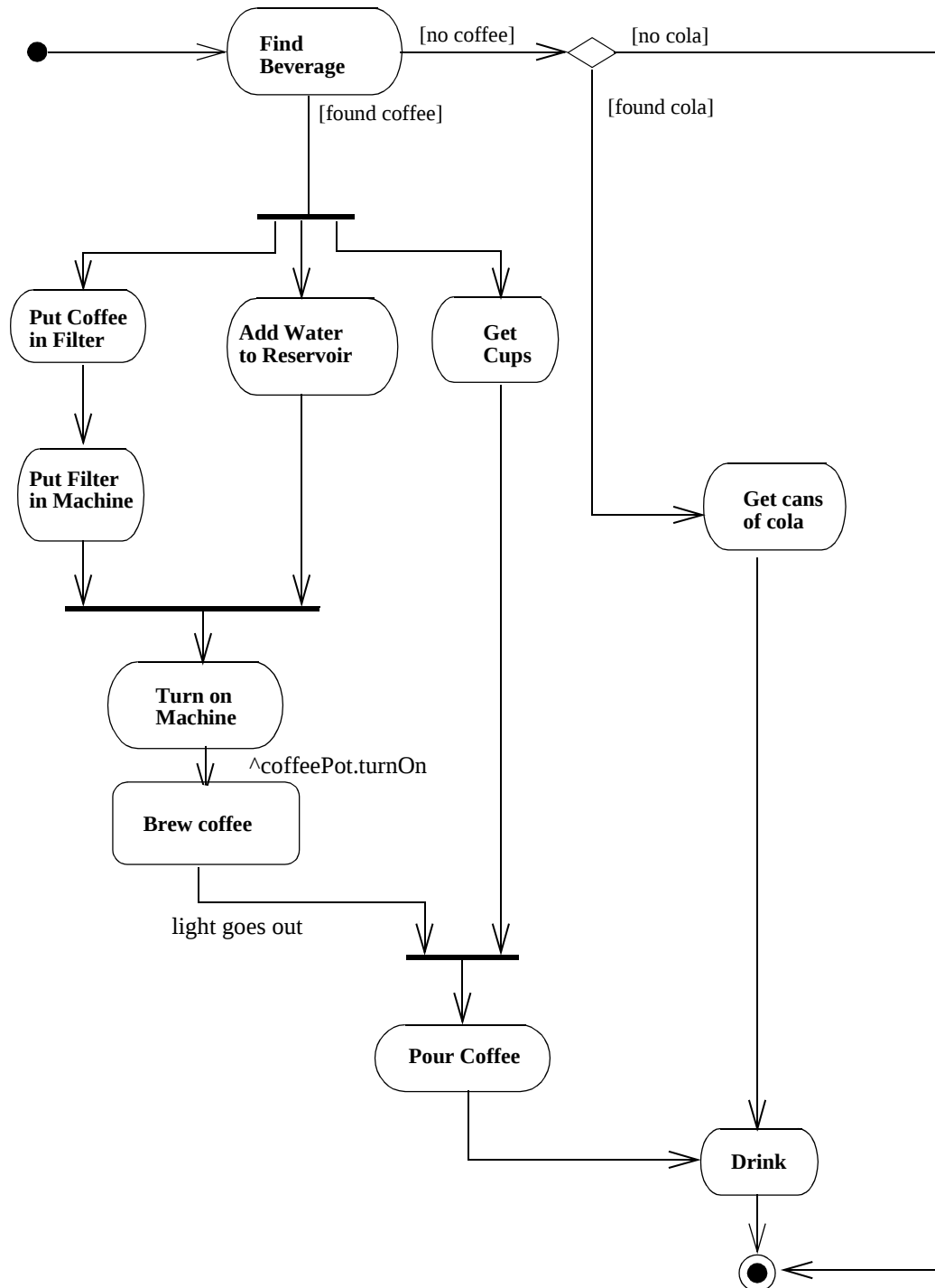
Figure 52. Activity diagram
