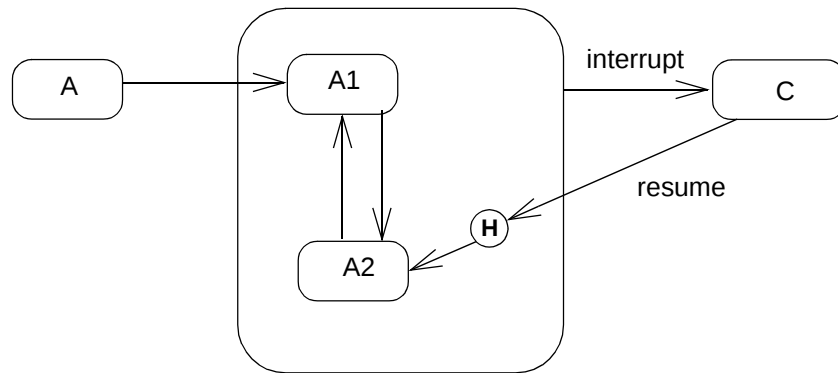
Figure 48. History indicator
