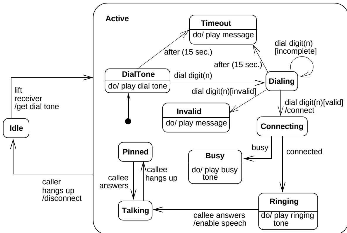
Figure 41. State diagram
