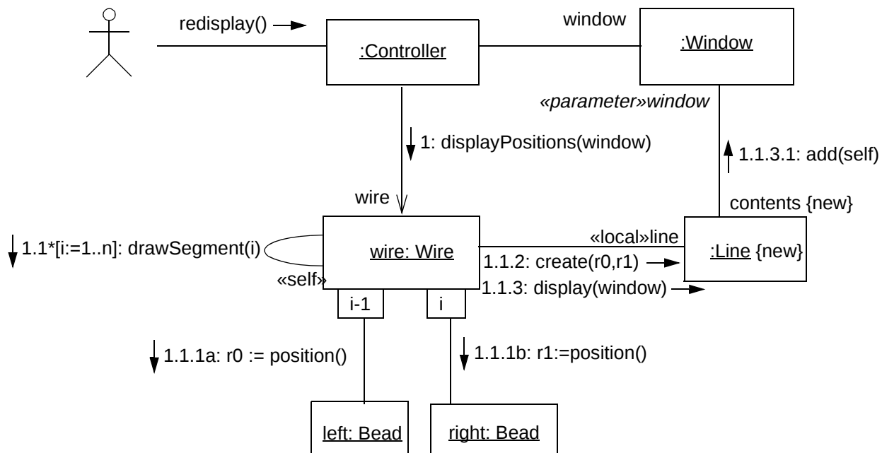
Figure 37. Collaboration diagram
