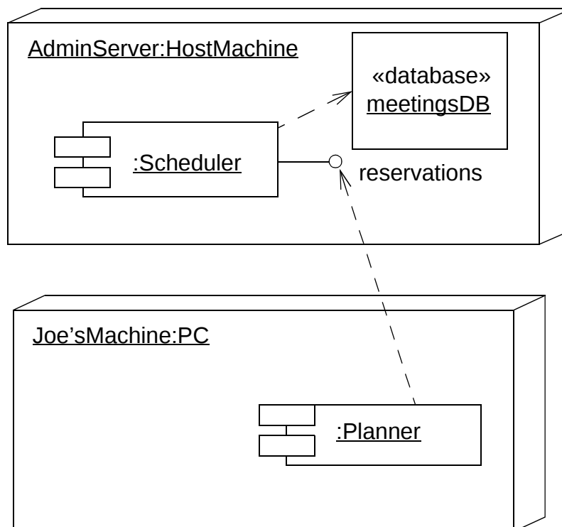
Figure 60. Nodes
