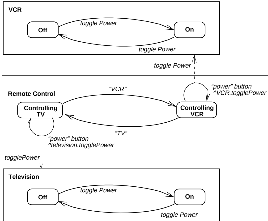
Figure 49. Sending messages
