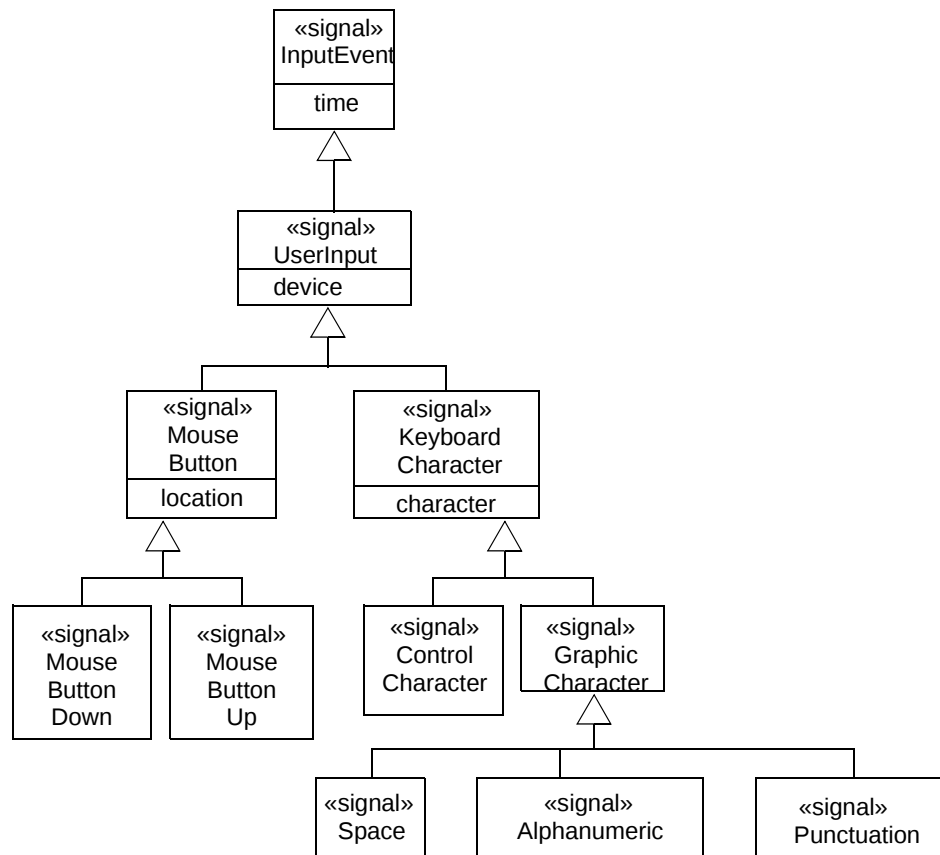
Figure 45. Signal declaration
