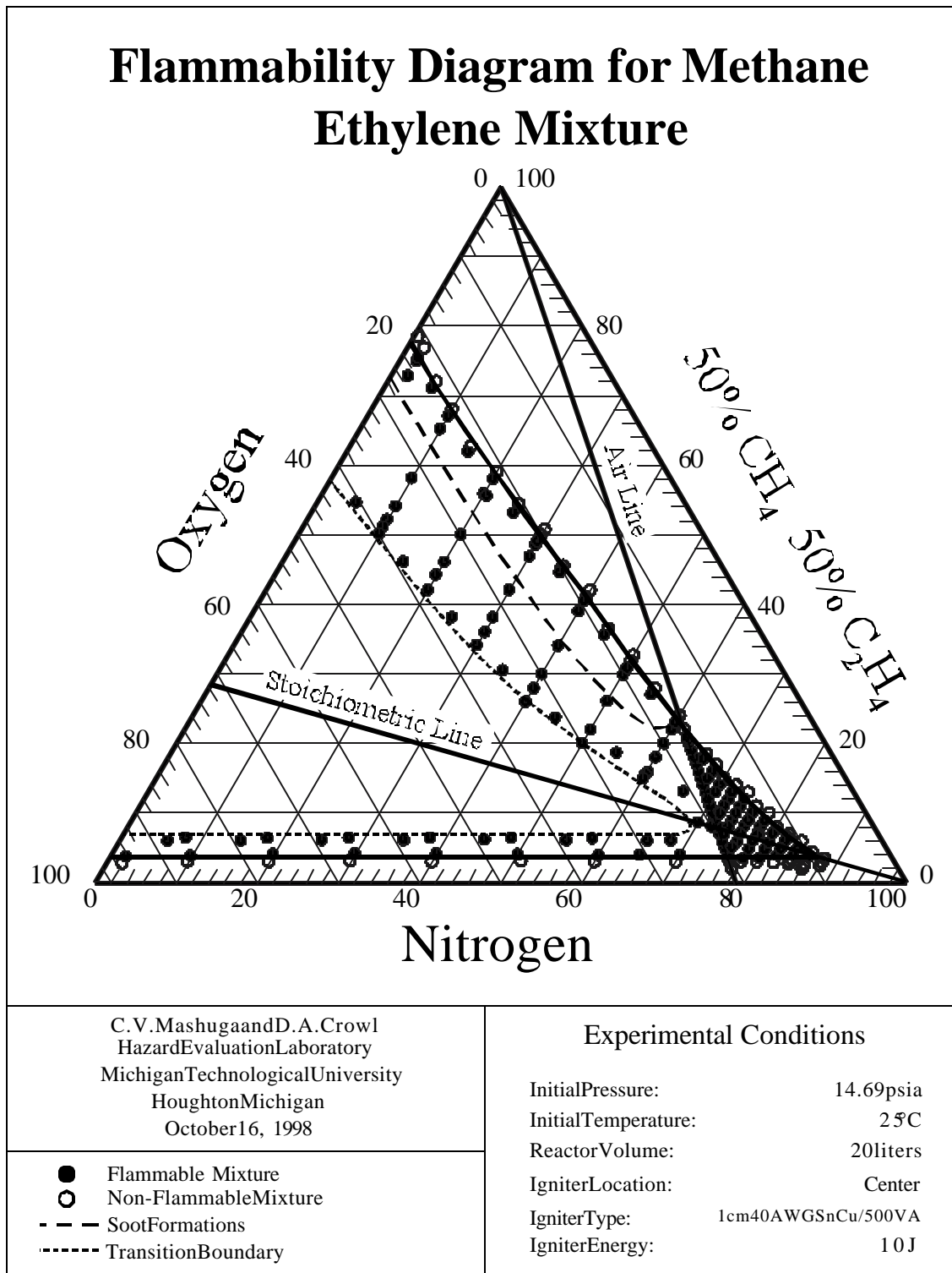
Figure 5.15: Experimental flammability diagram for 50/50 methane/ethylene mixture.
