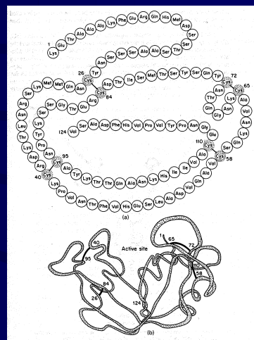
Figure 3-17. Structure of the enzyme ribonuclease. (a) Primary amino acid sequence.
