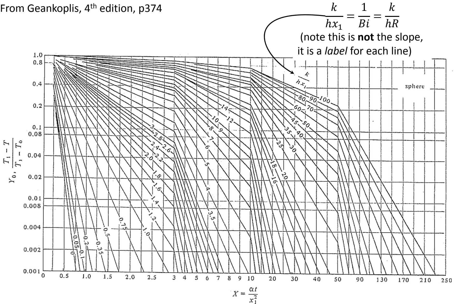
FIGURE 5.3-10. Chart for determining the temperature at the center of a sphere for unsteady-state heat conduction. [From H. P. Heisler, Trans. A.S.M.E., 69, 227 (1947). With permission.]
