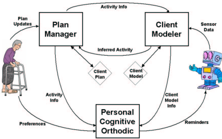
Figure 2: Autominder Architecture
