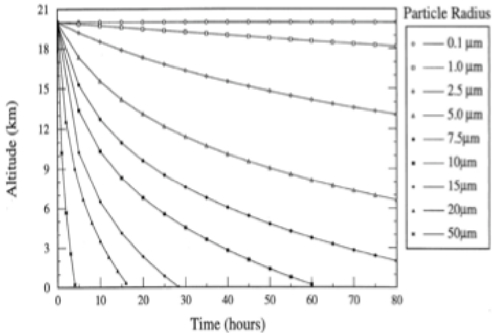
Figure 3. Fall distances for spherical, 0.1-50 \mu\text{m} radius, volcanic ash particles as a function of time. The local viscosity was determined from a radiosonde temperature profile collected at Veracruz, Mexico (380 km NW of El Chichón) on April 5 at 0000 UT.
