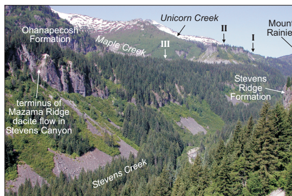
Figure B-9. Stevens Creek canyon from Stevens Canyon Road. The Mazama Ridge dacite flow of Stevens Canyon was dated by Sisson and Lanphere (1999) at about 90 ka. The direction of lava movement was upper right to lower left. Lescinsky and Sisson (1998) concluded that the flow was ponded at successively lower levels by tributary glaciers from the valleys of Unicorn Creek (bench level I, in the distance) and Maple Creek (bench level II) before being deflected and flowing downvalley at a lower elevation (bench level III in center and at left). The uppermost bench level is named 'The Bench'. View is to the west.
