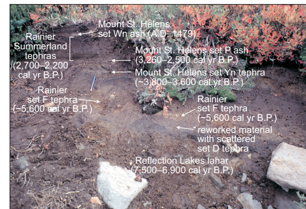
Figure B-4. Ash layers and buried soils overlying a lahar in Paradise Valley near the Fourth Crossing Trail parking area. USGS geologist Jim Vallance suggests that this lahar, which is likely the same one that underlies Reflection Lakes, dates to between 7,500 and 6,900 cal yr B.P., based on the ages of constraining tephra layers (written commun., 2002). Vallance also contributed the interpretations of the various tephra layers shown. He identified four 'exotic' (that is, not from Mount Rainier) tephra layers including Yn (3,800–3,600 cal yr B.P.), Wn (A.D. 1479), and set P (3,260–2,500 cal yr B.P.) tephra from Mount St. Helens. Mount St. Helens X tephra (~A.D. 1500) is present atop the Wn but is not visible in the photo. The blue pencil provides scale.
