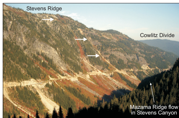
Figure B-8. Stevens Canyon and Stevens Ridge from about 1 mi (1.6 km) east of Lake Louise. Arrows at top and center show the approximate contact of Tatoosh granodiorite (left; 25.8–14.1 Ma) with the welded tuffs of the Stevens Ridge Formation. Notice the differences in the vegetation growing on the respective rock units; the horizontal stripes to the right suggest bedding. Cowlitz Divide is composed of the Ohanapecosh Formation (~37–27 Ma). The Mazama Ridge flow is about 90 ka. View is to the east.
