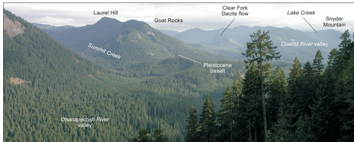
Figure B-16. View from Backbone Ridge to the southeast across the Ohanapecosh River valley at the Clear Fork Dacite flow and Goat Rocks (see Leg H, p. 124). Geoff Clayton (1983) obtained a radiometric age of about 0.65 ka on this flow. Hammond (1989) suggested that the Clear Fork flow may have been ponded by a lobe of ice in the upper Cowlitz River valley. The Pleistocene basalt shown might have been erupted from the Tumac Mountain volcano 10.5 mi (17 km) to the east or from a vent a few miles/kilometers west of Ohanapecosh valley along Summit Creek. Snyder Mountain is cored in large part by a thick pyroxene andesite lava flow erupted from Goat Rocks volcano between 0.78 and 0.14 Ma (Swanson and others, 1997). Swanson and his colleagues noted that the flows filled canyons incised as deep as 1150 ft (350 m) in upper Oligocene volcaniclastic rocks. A large debris avalanche from Snyder Mountain dammed upper Lake Creek to form Packwood Lake; the youngest radiocarbon age on a barkless snag in the lake is 970 yr B.P. (Pringle and others, 1998).
