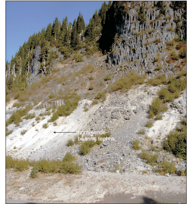
Figure B-7. The toe of Mazama Ridge where the Mazama Ridge lava flow (~99 ka; not shown) caps an older lava flow (columnar joints) over a lahar or pyroclastic flow over a hornblende-bearing tephra that is possibly correlative with the Sunset Amphitheater tephra (~190 ka). It is about 60 ft (18 m) to the base of the older lava flow. View is to the north.
