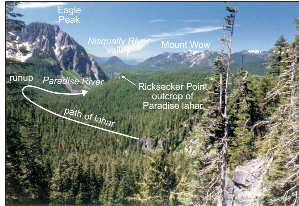
Figure B-6. The view west-southwest down Paradise Valley to Ricksecker Point from Inspiration Point. Ricksecker Point is the toe of a relatively young, fairly thick lava flow from Mount Rainier. That flow, whose age has been estimated at about 40 ka (Sisson and Lanphere, 1999), was probably ponded by glaciers that sat in the Paradise and Nisqually River valleys. The Paradise lahar sloshed through this valley about 5000 years ago, leaving a deposit at Ricksecker Point, some 800 ft (245 m) above the valley bottom (see Fig. A-23, p. 65). Eagle Peak and adjoining peaks of the Tatoosh Range to the west are cored by intrusive granodiorite of the Tatoosh pluton (25.8–14.1 Ma) and capped by older welded tuffs and breccias of the Stevens Ridge Formation.
