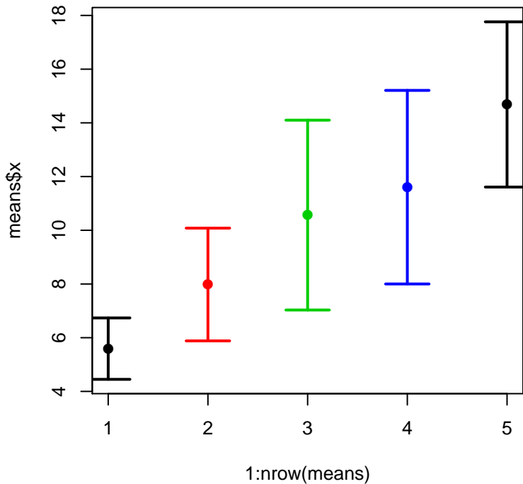
plotrix plotCI with additions
