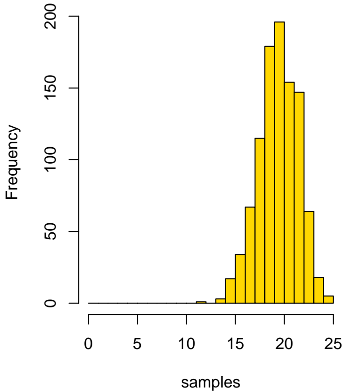
Histogram of samples
