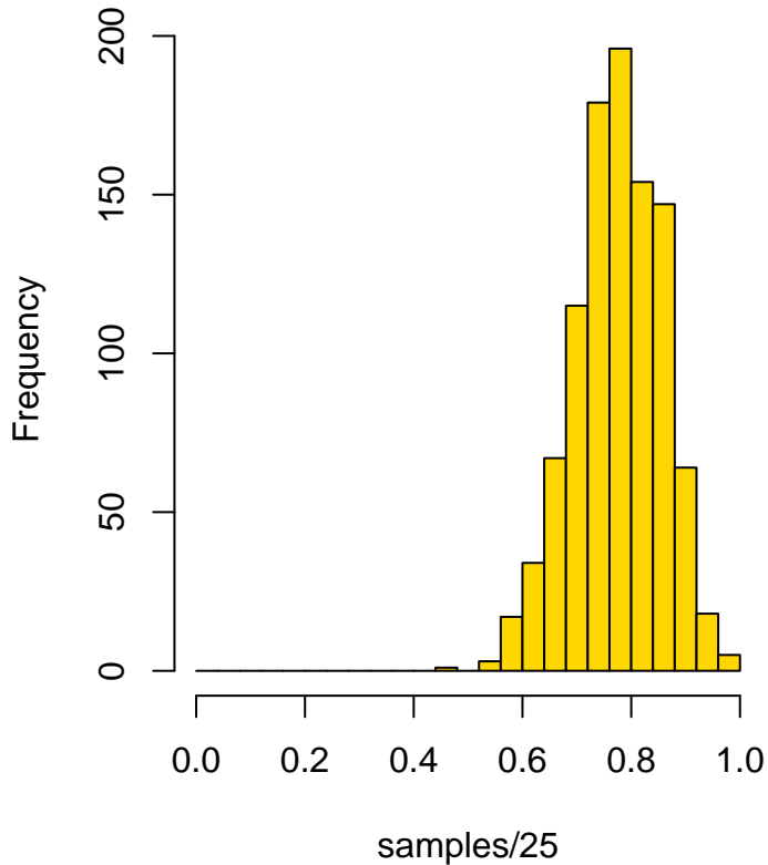
Histogram of samples/25
