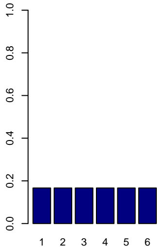
Die Roll Probability Density
