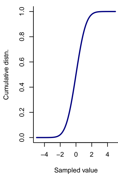
Normal Random Variable Cumulative distribution
