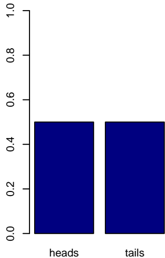
Coin toss Probability Density
