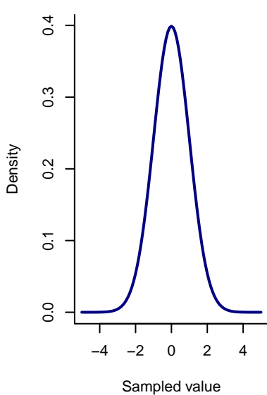
Normal Random Variable Probability density
