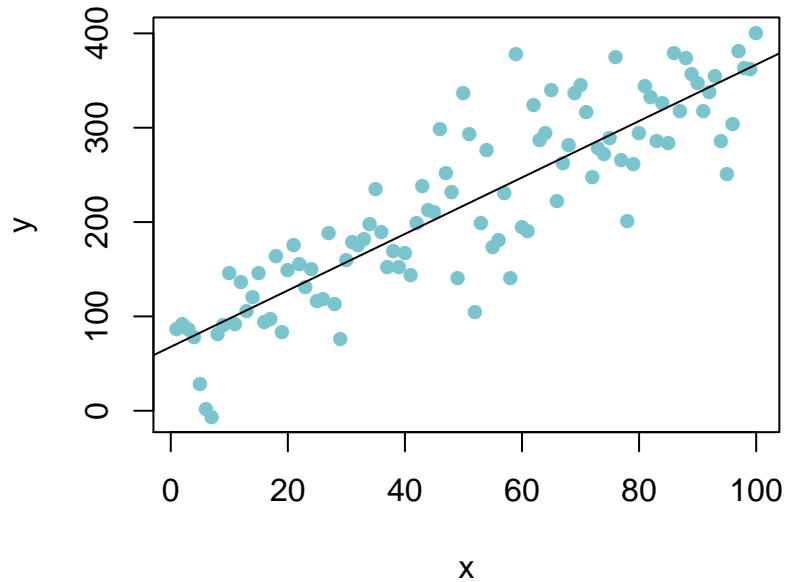
Data and predicted model with some noise
