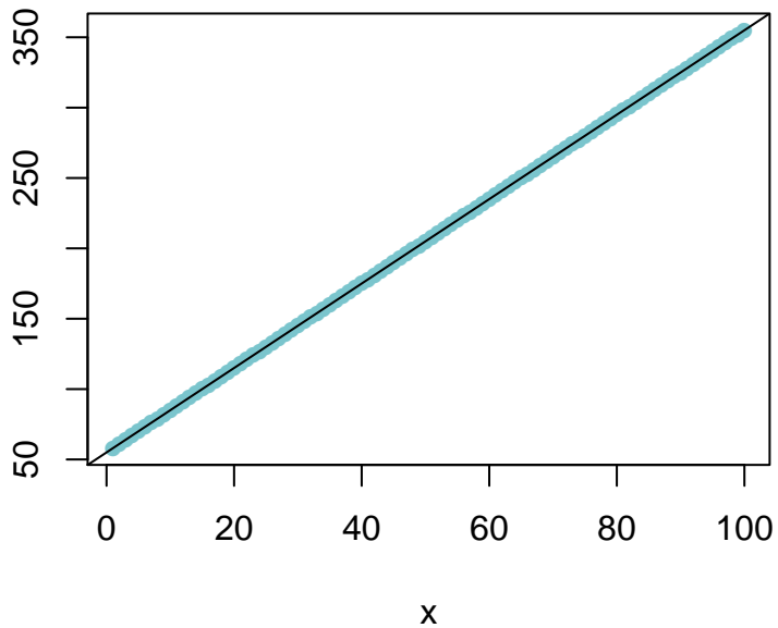
Data and predicted model with no noise
