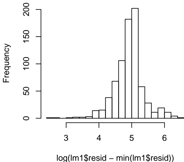
Histogram of log(lm1$resid - min(lm1$resid))
