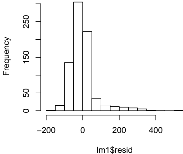
Histogram of lm1$resid
