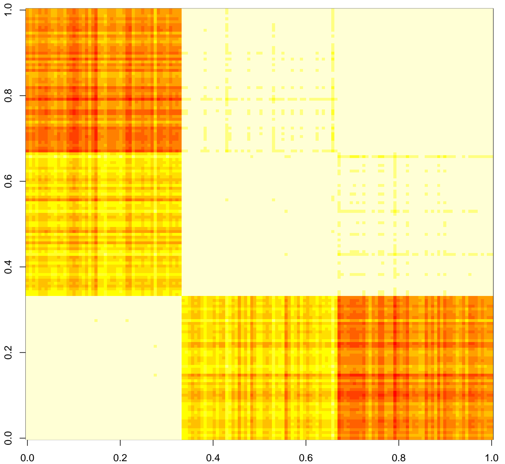
Correlation map of iris data
