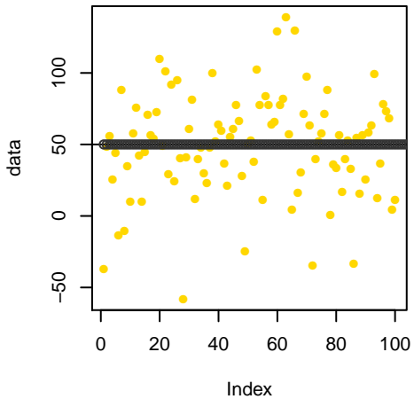
Mean=50, StdDev=0
