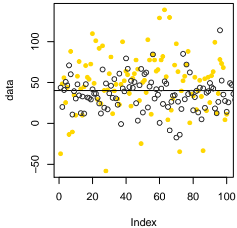
Mean=40, StdDev=20
