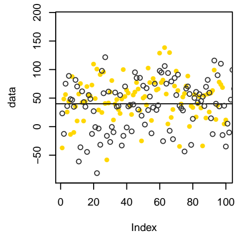
Mean=40, StdDev=40
