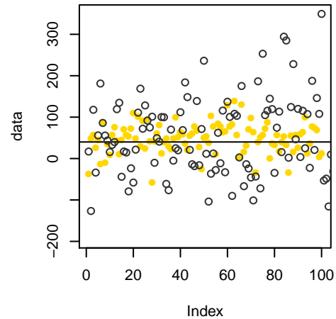
Mean=40, StdDev=40
