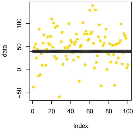
Mean=40, StdDev=0
