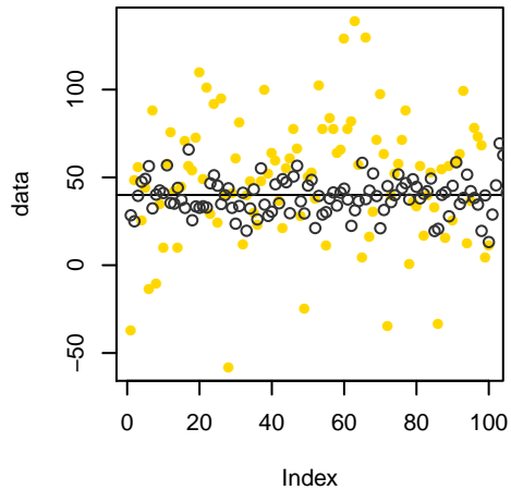
Mean=40, StdDev=10
