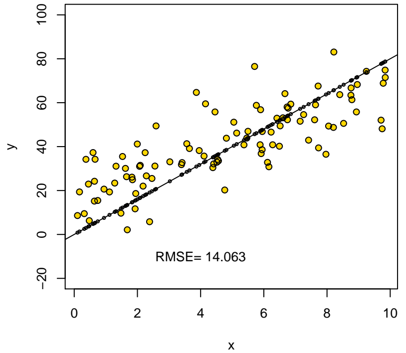
intercept: 0 slope: 8
