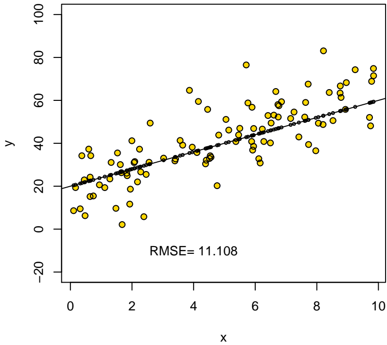
intercept: 20 slope: 4
