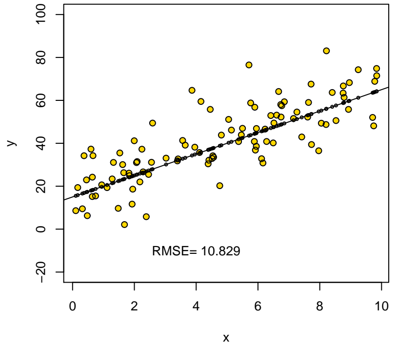
intercept: 15 slope: 5
