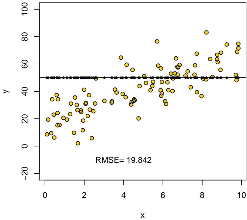
intercept: 50 slope: 0
