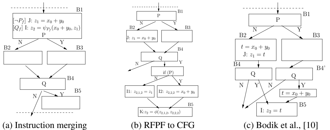
Figure 8.2: Merging and Converting Back to CFG
