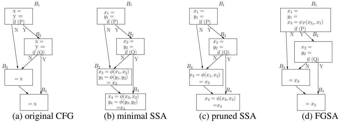
Figure 3.1: An FGSA Example
