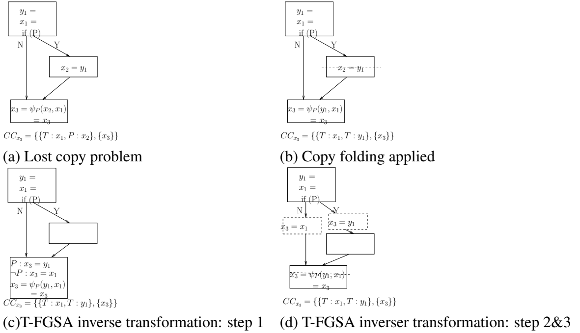
Figure 5.1: Translation from FGSA
