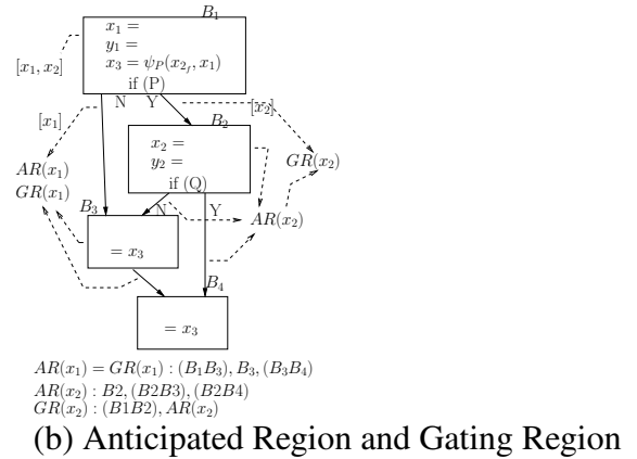
Figure 4.5: Extended liveness on FGSA
