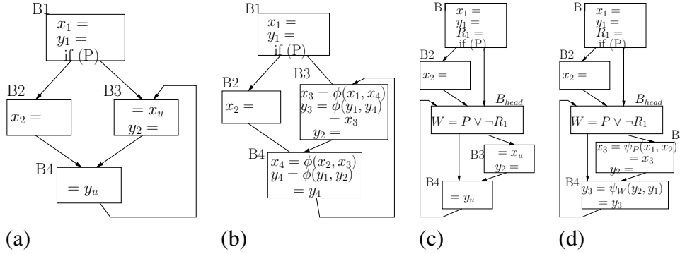
Figure 3.8: T_R transformation on an irreducible graph
