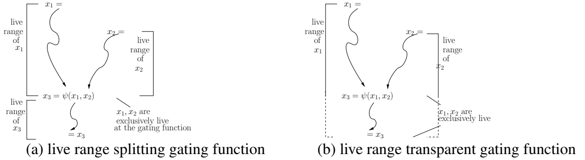
Figure 4.3: Two liveness approaches in general single assignment form
