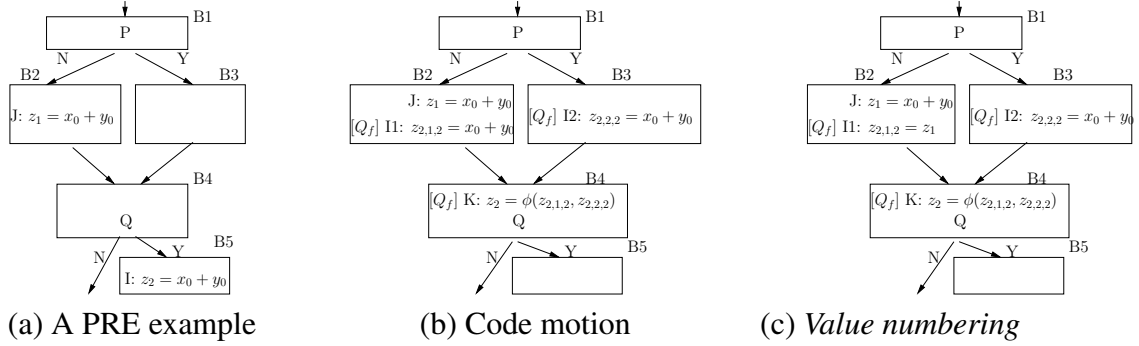
Figure 8.1: Partial redundancy elimination during the code motion
