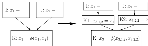
Figure 7.4: \phi -node elimination
