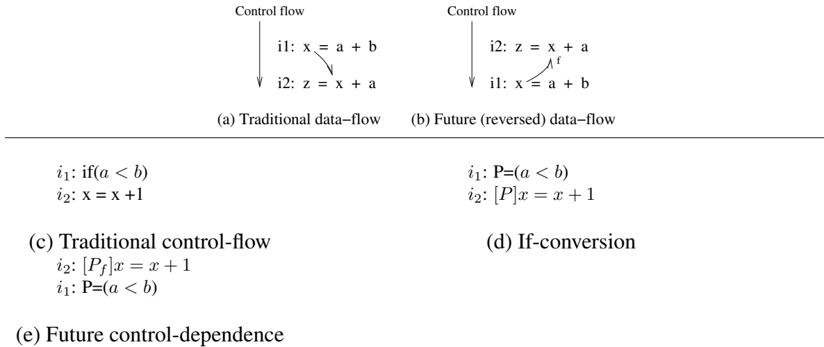
Figure 2.6: The concept of future data and control dependencies
