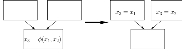
Figure 2.3: Insert copy assignments to eliminate a \phi -function
