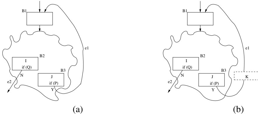
Figure 7.8: Theorem 7.3.1
