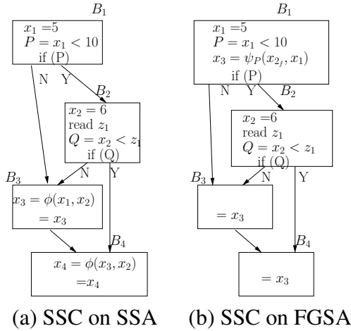
Figure 6.2: Constant propagation
