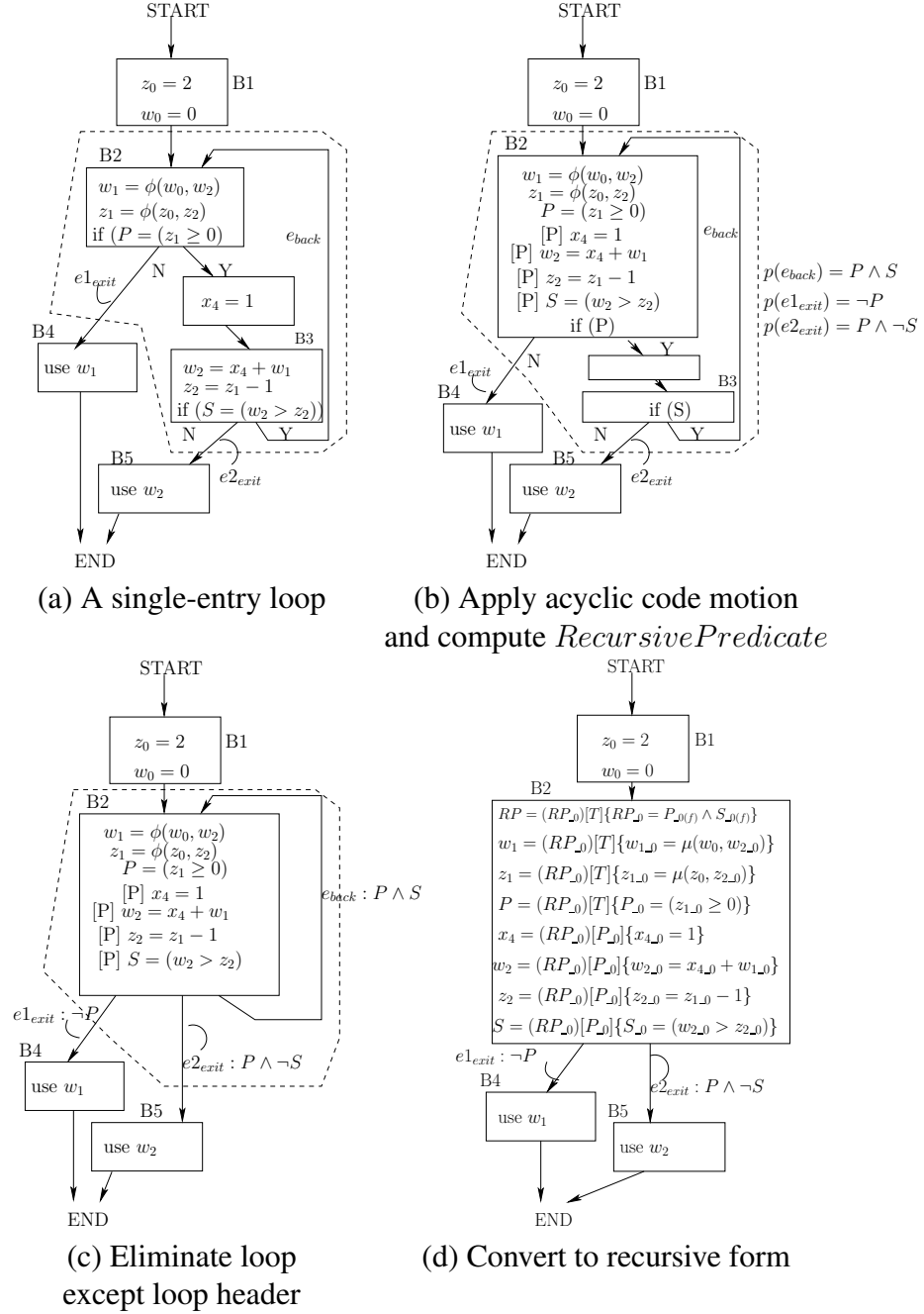
Figure 7.9: Program 1: Conversion of a cyclic program into RFPF
