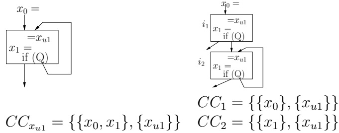
Figure 3.2: A non-path-separable CC: use belongs to two CCs
