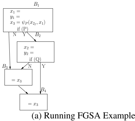
Figure 4.5: Extended liveness on FGSA
