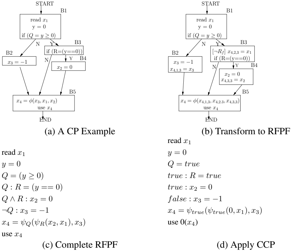
Figure 8.3: Constant propagation on RFPF
