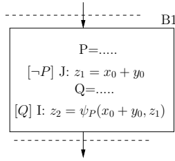
Figure 8.1: Partial redundancy elimination during the code motion
