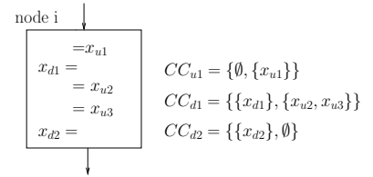
Figure 3.3: Local CCs computation
