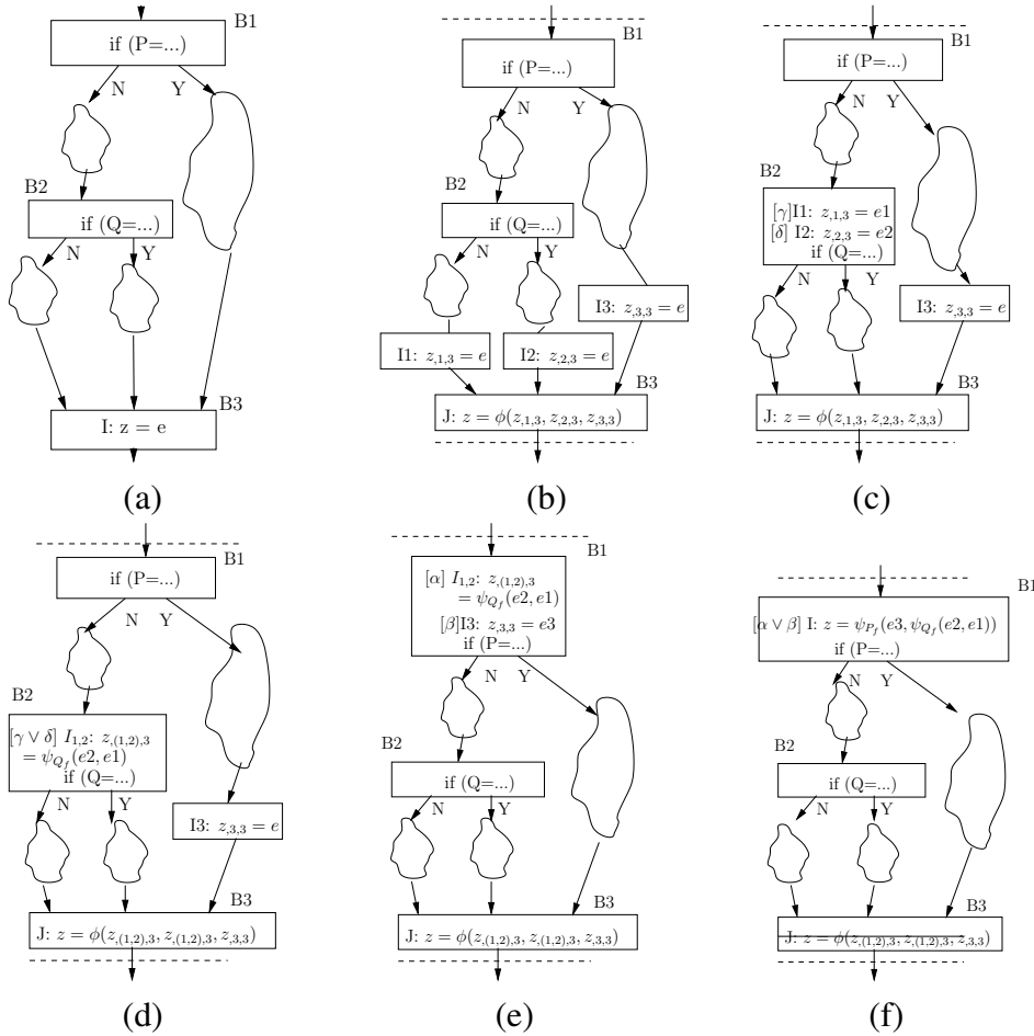
Figure 7.6: Instruction merging
