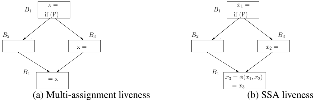
Figure 4.1: Traditional liveness
