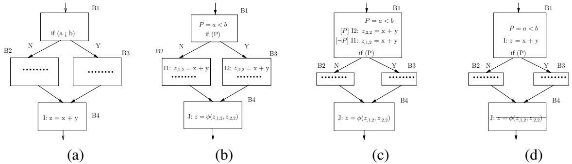
Figure 7.5: Instruction propagation
