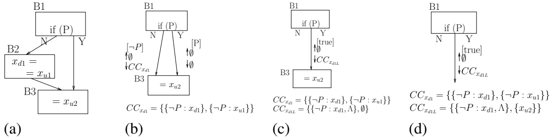
Figure 3.4: T2 example
