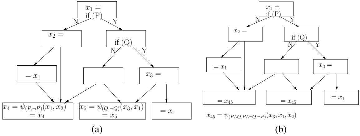
Figure 5.9: Common use form
