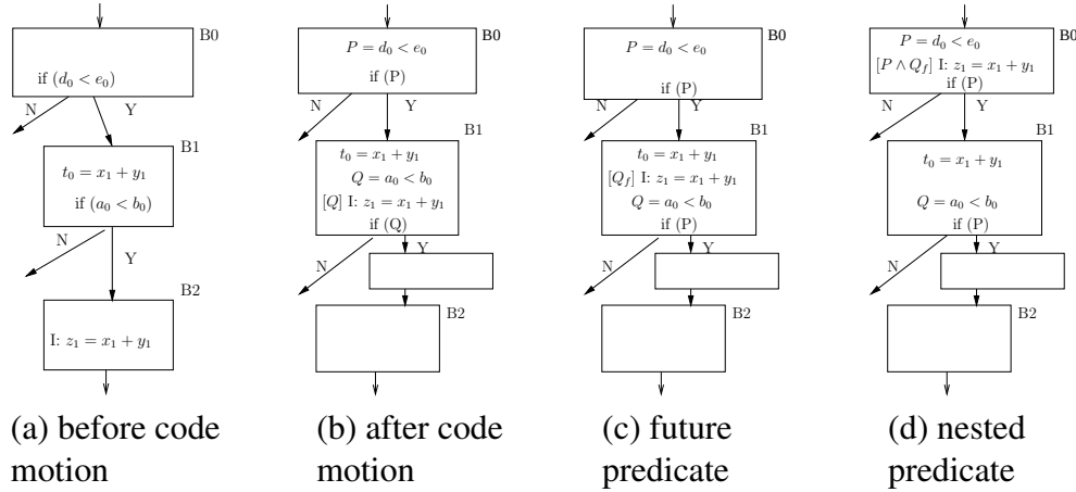
Figure 7.3: Code motion across control dependent regions
