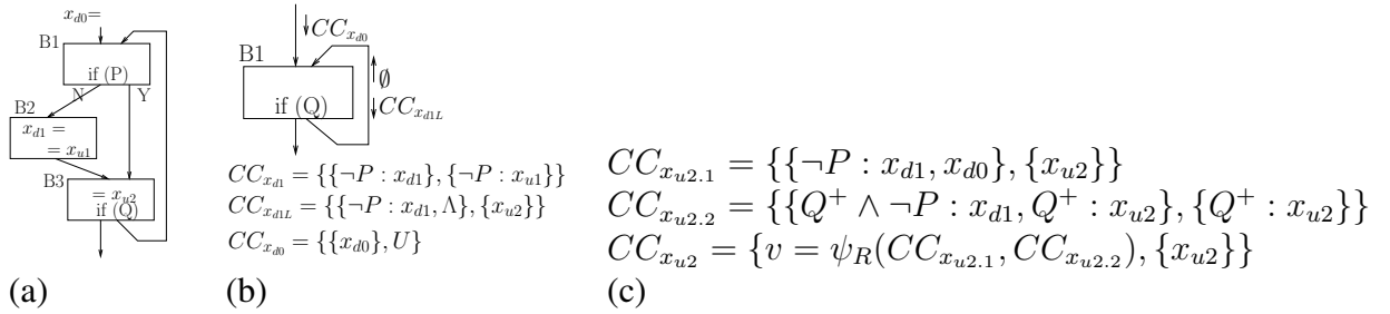
Figure 3.7: A self-referencing gating function
