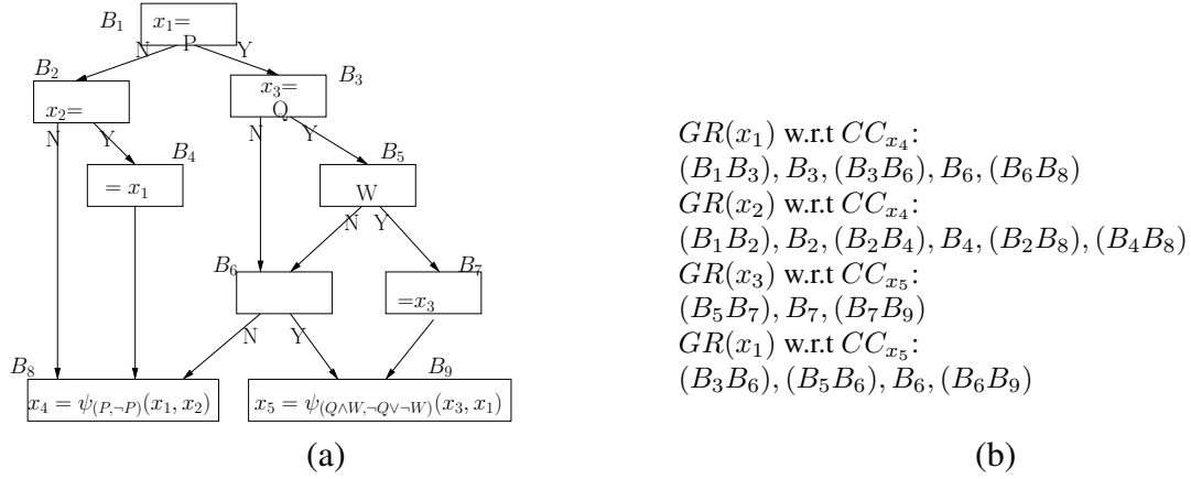
Figure 4.6: Gating region
