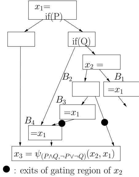
Figure 5.6: Interferences of uses in different regions
