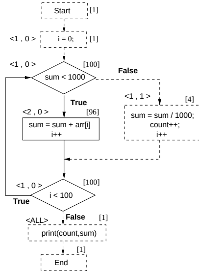
(b) Power-aware flow graph.
