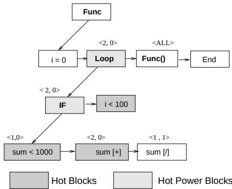
(c) Hierarchical tree with power blocks.
