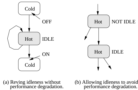
Fig. 3. Idleness removal strategy.
