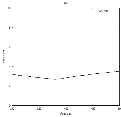
(e) sor 2×4K Color
