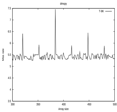
(g) dmxpy 8K Traditional
