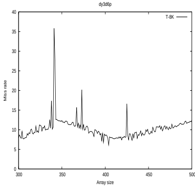
(a) dy3d6p 8K Traditional
