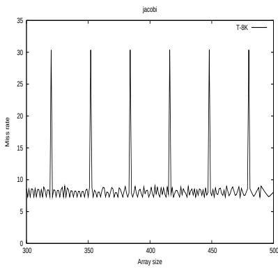
(g) jacobi 8K Traditional
