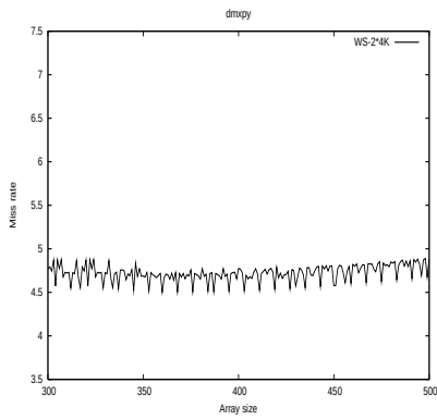
(h) dmxpy 2x4K Color
