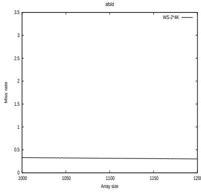
(b) afold 2x4K Color
