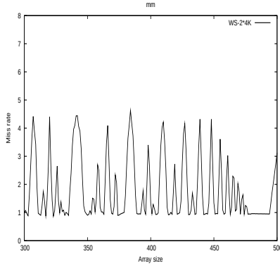
(b) mm 2×4K Color
