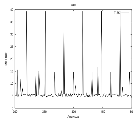
Figure 1: Miss Rates of Tiled Loop
