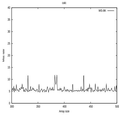
(e) calc 2x4K Color
