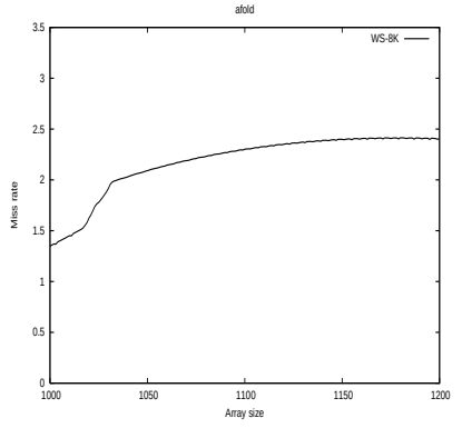
(c) afold 1x8K Color
