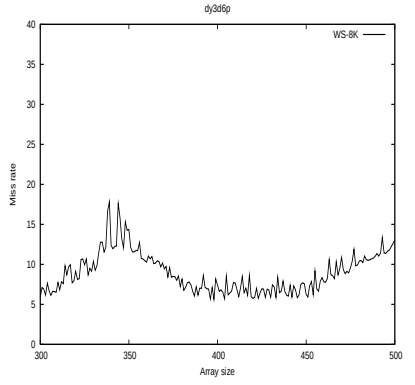
(c) dy3d6p 1 \times 8K Color
