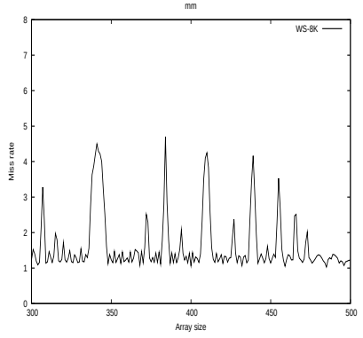
(c) mm 1×8K Color
