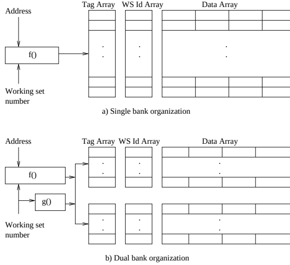
Figure 5: Cache organizations
