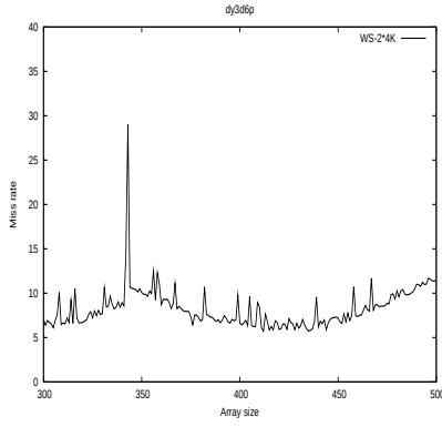
(b) dy3d6p 2 \times 4K Color
