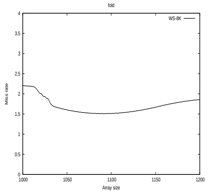
(f) fold 1 \times 8K Color
