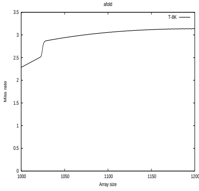
(a) afold 8K Traditional
