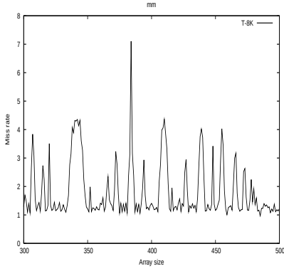
(a) mm 8K Traditional
