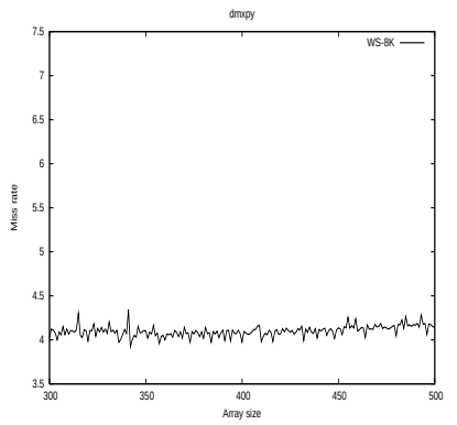
(i) dmxpy 1x8K Color
