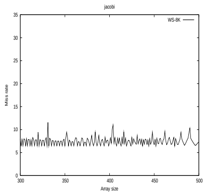
(i) jacobi 1 \times 8K Color
