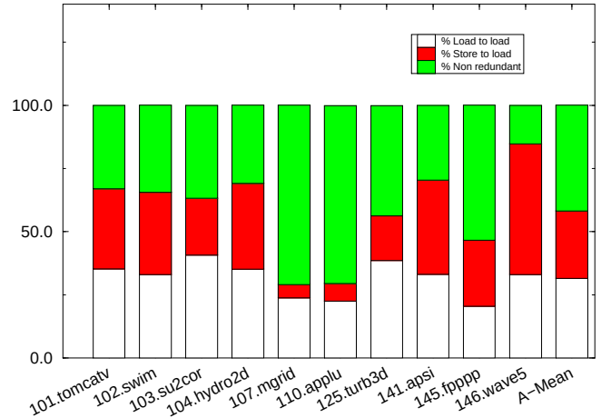
Figure 8: SPECfp95 - Load-to-load forwarding: store-to-load forwarding: non-redundant loads
