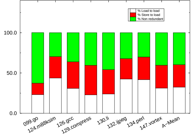
Figure 7: SPECint95 - Load-to-load forwarding: store-to-load forwarding: non-redundant loads
