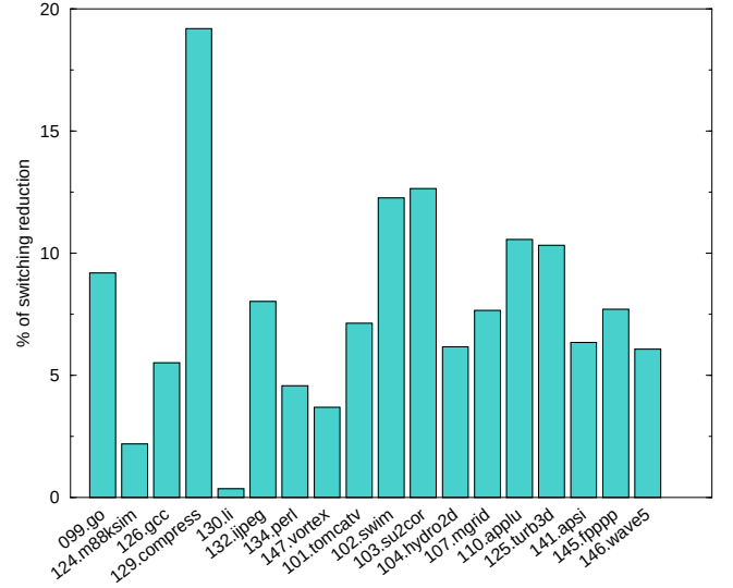
Figure 15: SPEC95 - reduction in switching.
