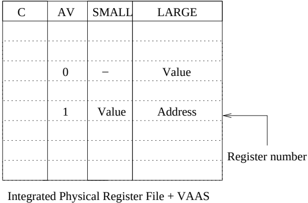
Figure 4: Restricting optimizations to small values.
