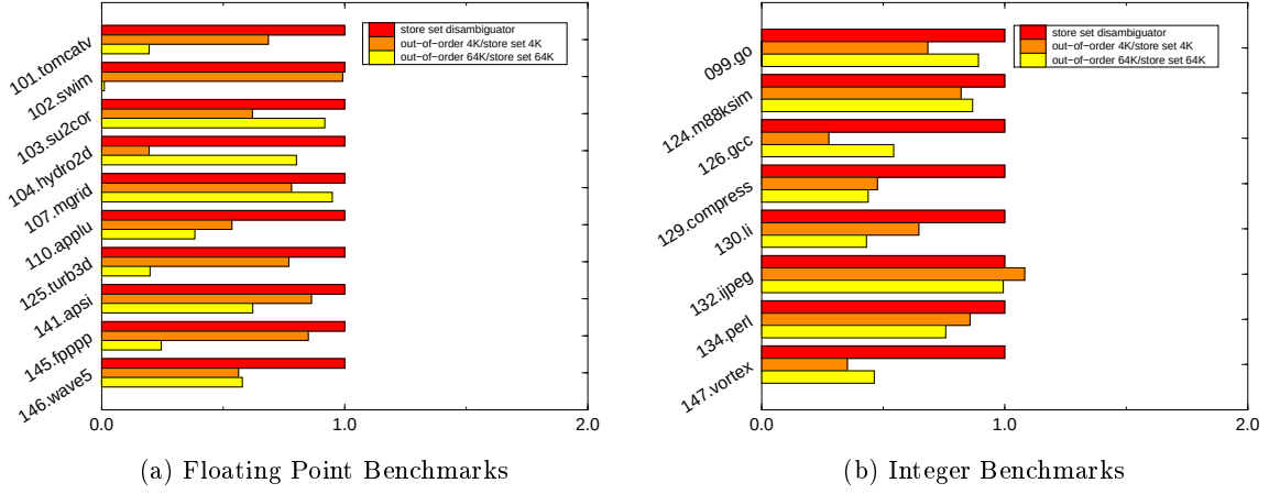
Figure 14: Normalized False Memory Dependencies
