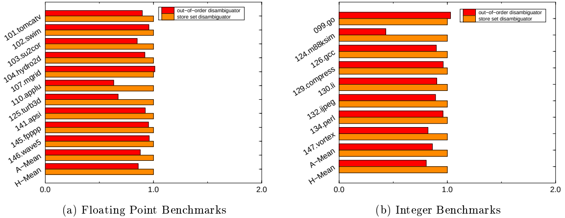
Figure 15: Normalized Counts of Load/Store Instructions Synchronized Via SSIT Table
