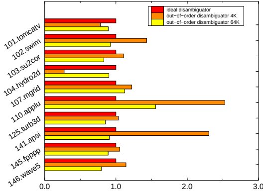
(a) Floating Point Benchmarks
