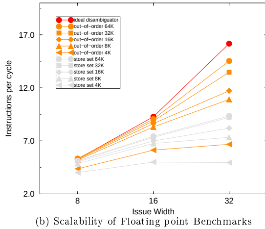
Figure 5. Scalability of Out-of-order Algorithm
