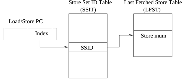
Figure 1. Store Set Implementation
