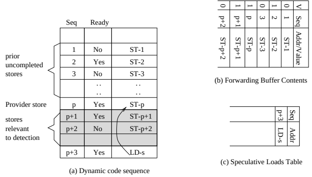
Figure 4. Speculative issuing of loads
