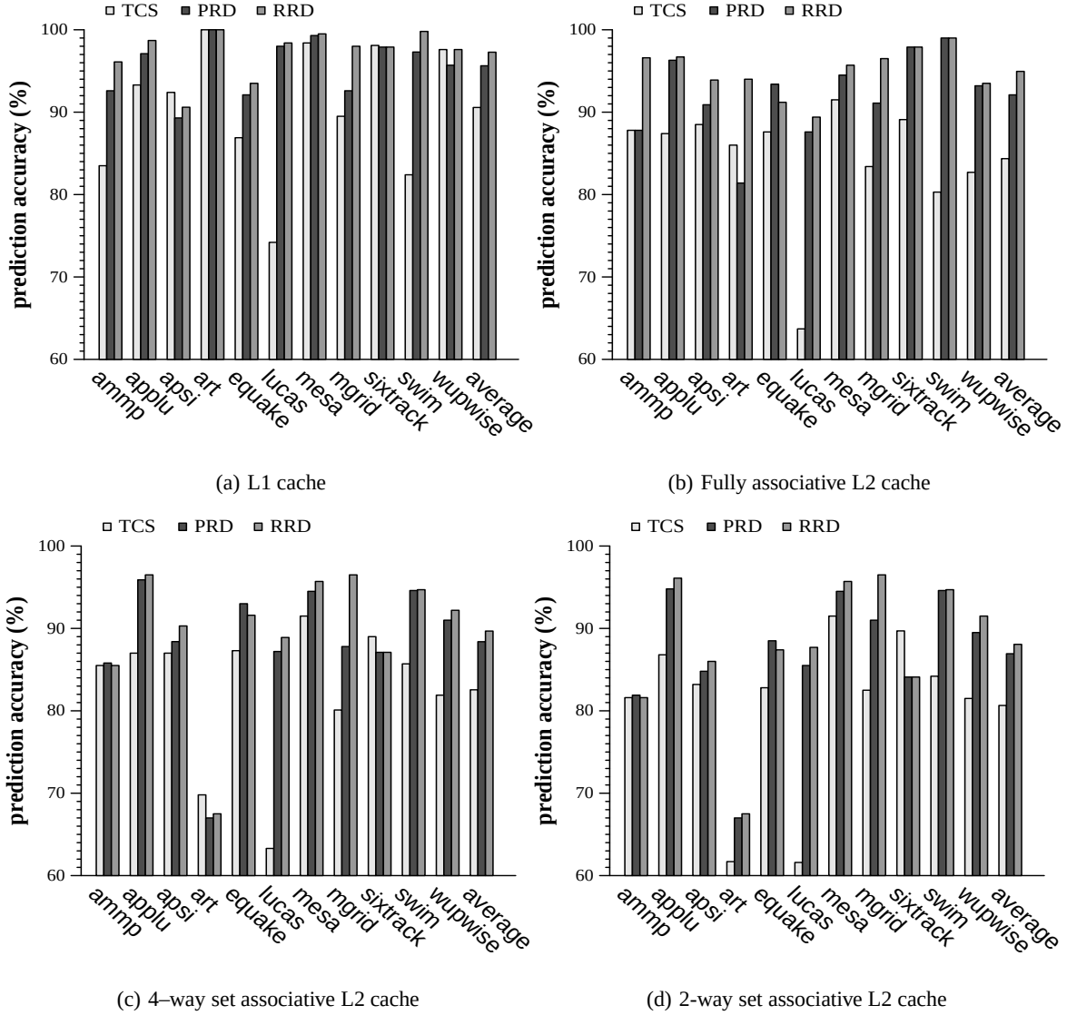
Figure 1: Dynamic miss-rate prediction accuracy
