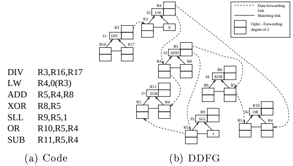
Figure 4. Sample code and its DDFG
