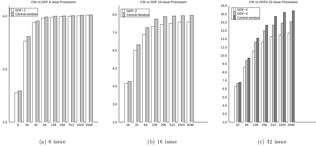
Figure 6. IPC values for DDFA and CW
