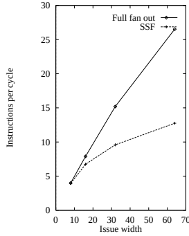
Figure 3. SSF-2 versus full fanout
