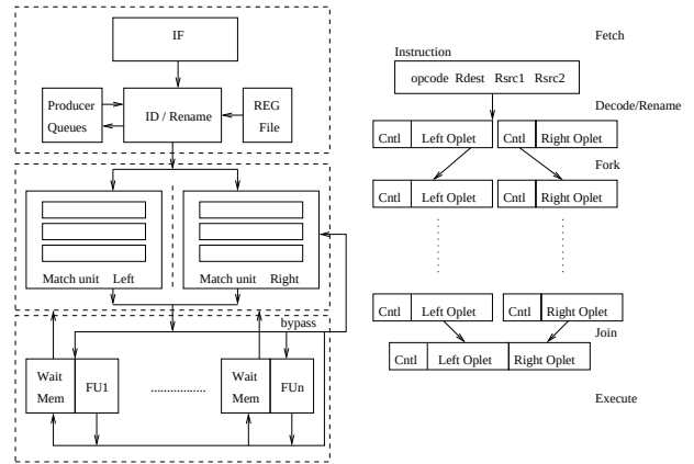
Figure 5. Superscalar Dynamic Data Forwarding Architecture (DDFA)
