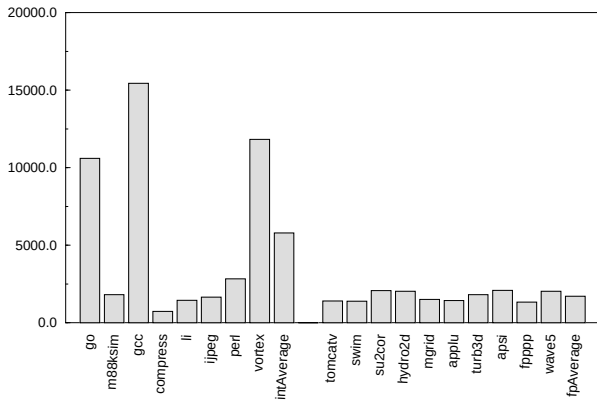
Figure 4. Maximum number of instructions stored in the sequence table.
