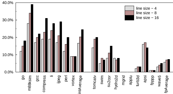
Figure 3. Percentage reduction in cache lines fetched.
