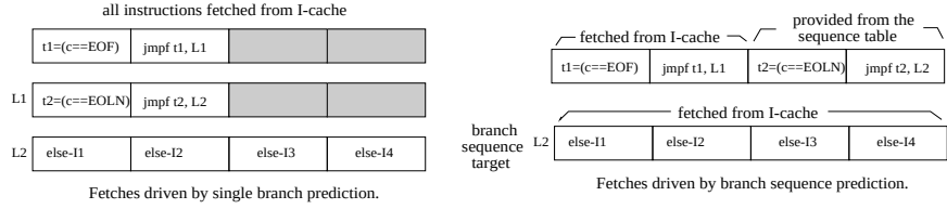
Figure 1. An example of a branch sequence.
