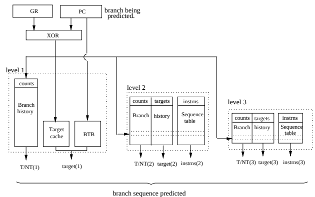
Figure 8. Branch sequence predictor.
