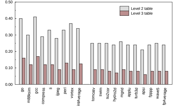
Figure 6. Expected sizes of second and third level tables relative to the first level table.
