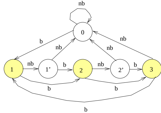
Figure 9. Sequence detection and history update.
