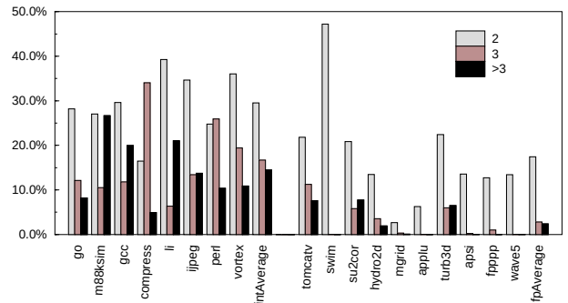
Figure 5. Percentage of branches in sequences of length 2, 3 and >3.
