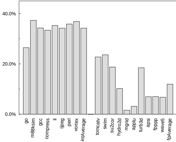
Figure 2. Dynamically executed branches that can benefit from branch sequence prediction.
