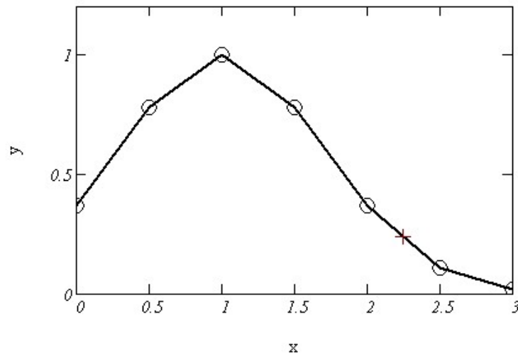
Figure 2. Linear interpolation lines. The circles (o) are the data points given in Table 1, while the cross (+) symbol represents the interpolated point for x = 2.25 .
