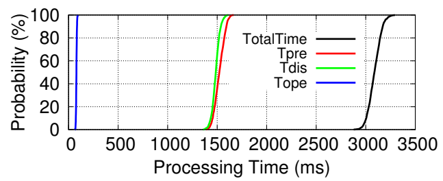
Fig. 13: The CDF of the ID claim/revocation arbitration time.
