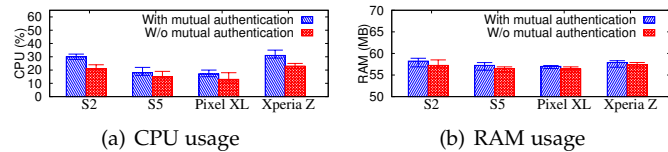
Fig. 11: The peak CPU and RAM usage statistics (max/med/min) of the MPKIX-enabled phones for the ppQuery service.
