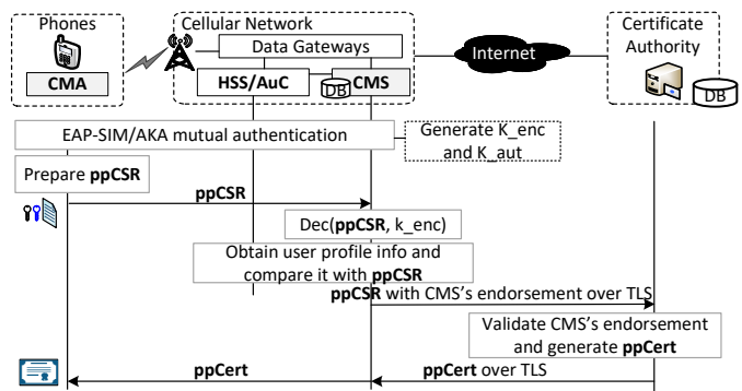
Fig. 3: MPKIX carrier-endorsed user certificate issuance.
